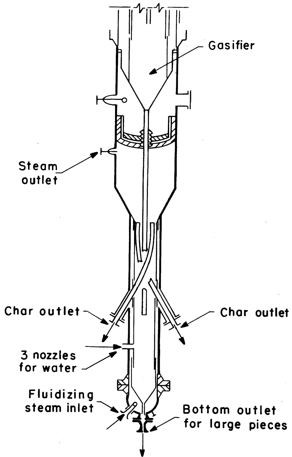
FIGURE 8. - Char Cooler.
