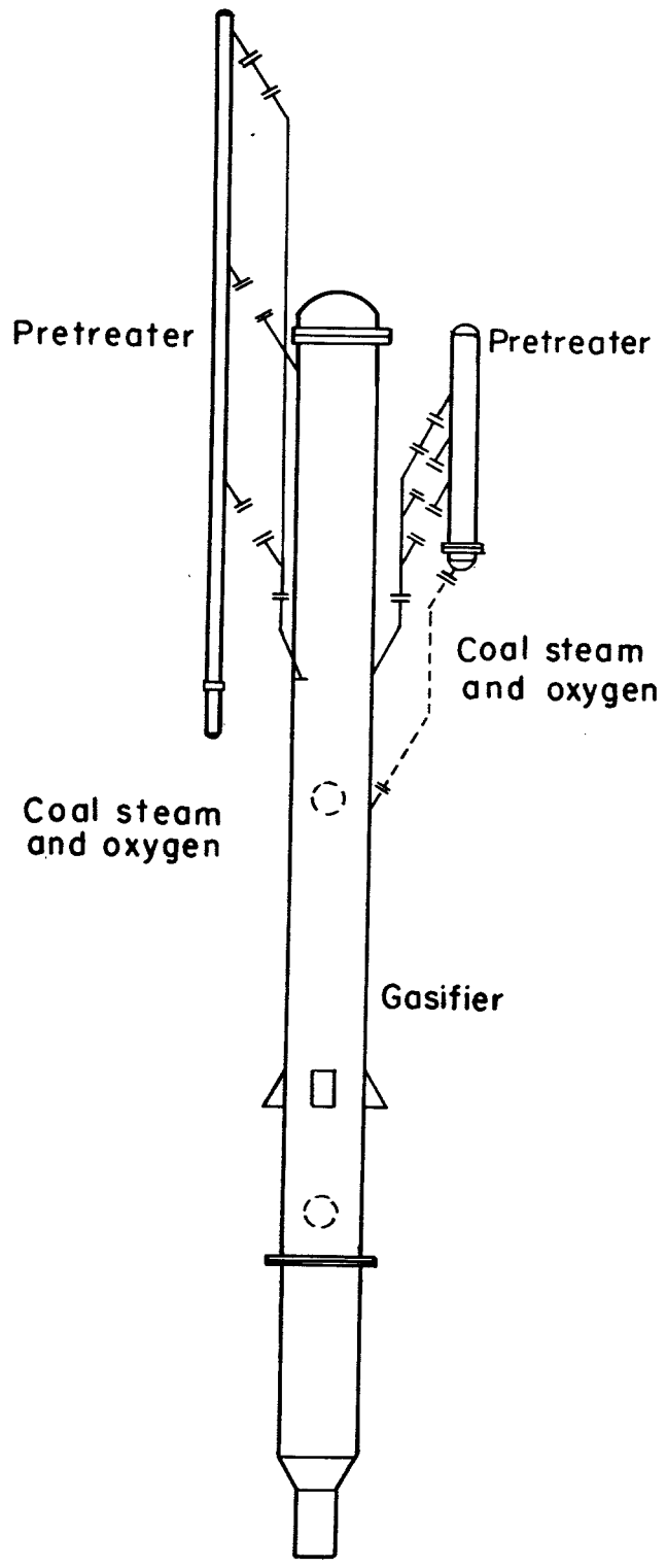
FIGURE 6. - Pretreater and Gasifier (Prototype).
