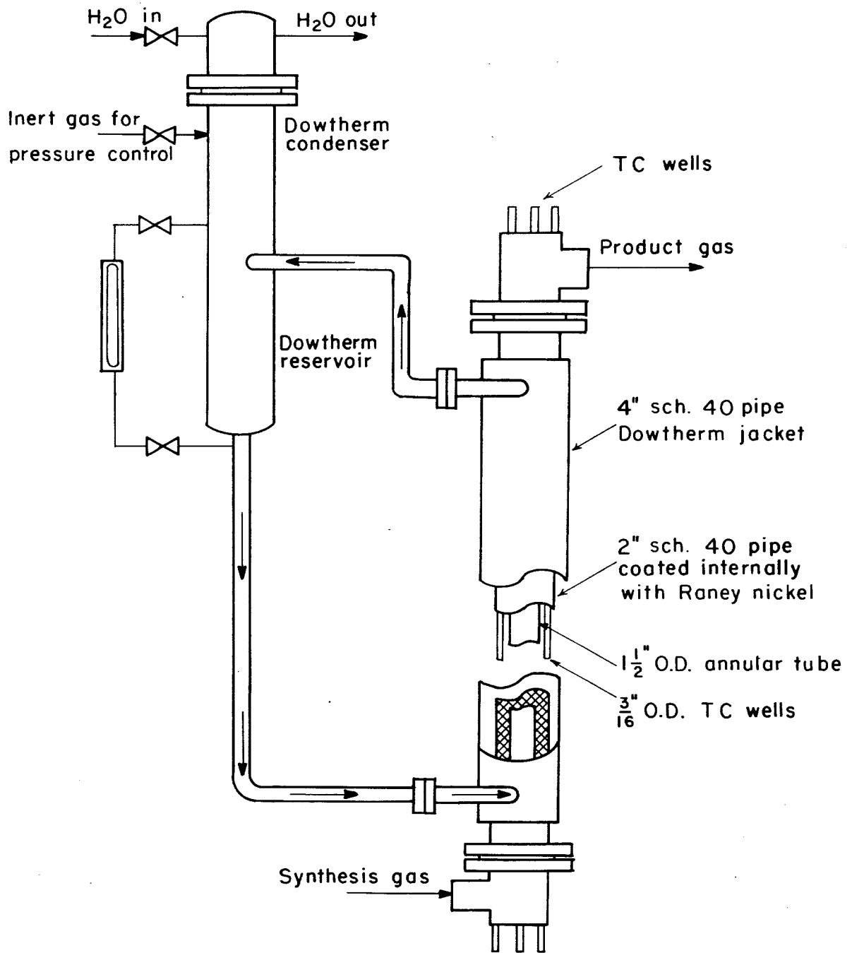
FIGURE 3. - Synthane Process Pilot Plant Methanation Reactor.
