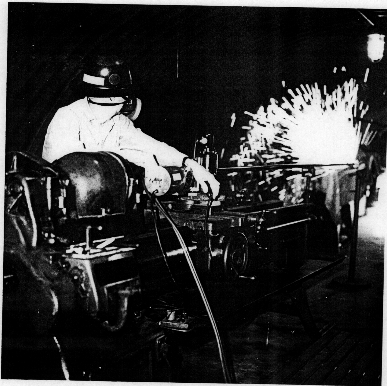
FIGURE 12. - Gun Used to Spray 2-inch Diameter Tubes Internally.
