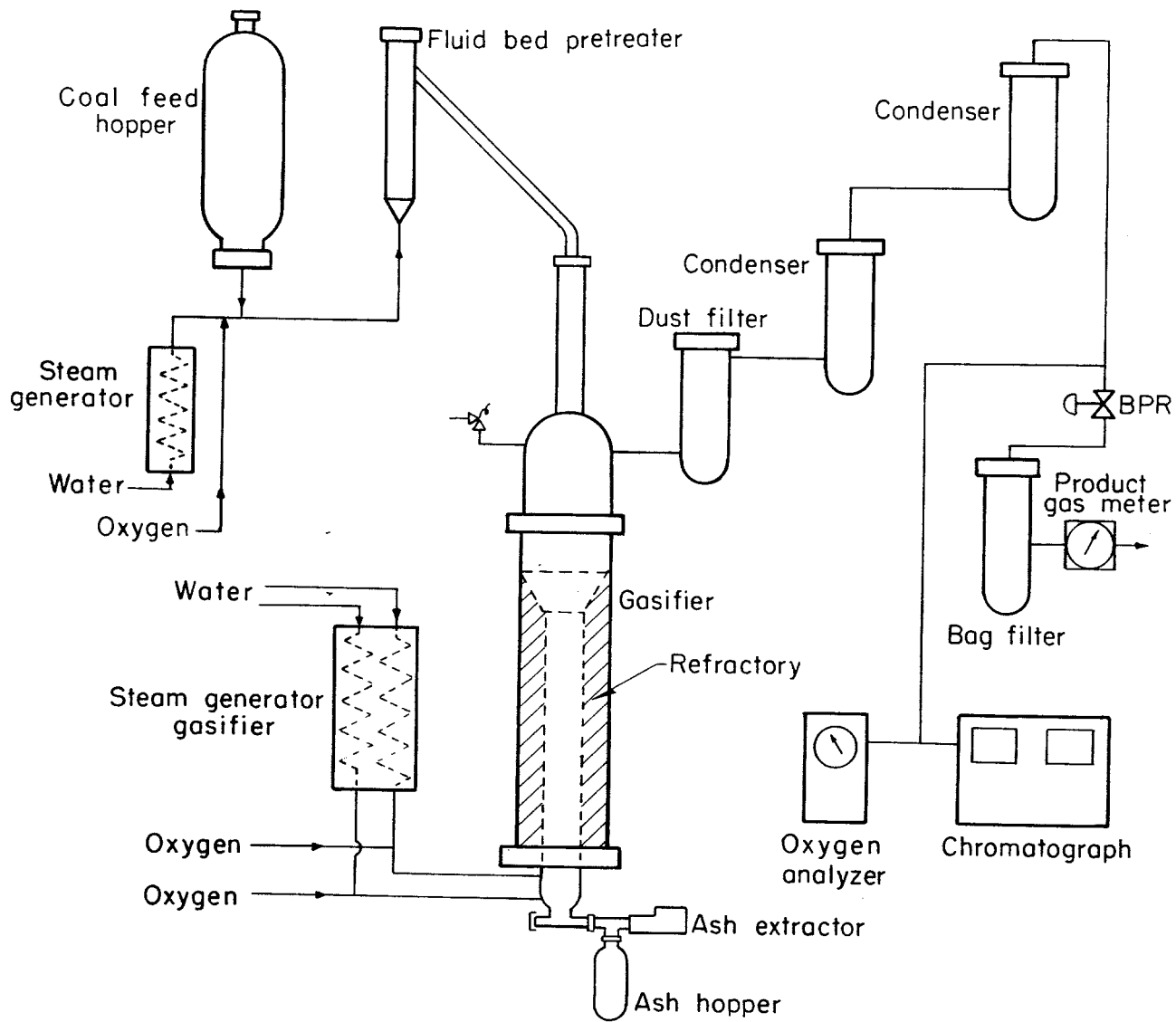
FIGURE 1. - 40 Atmosphere Fluid-Bed Gasifier.
