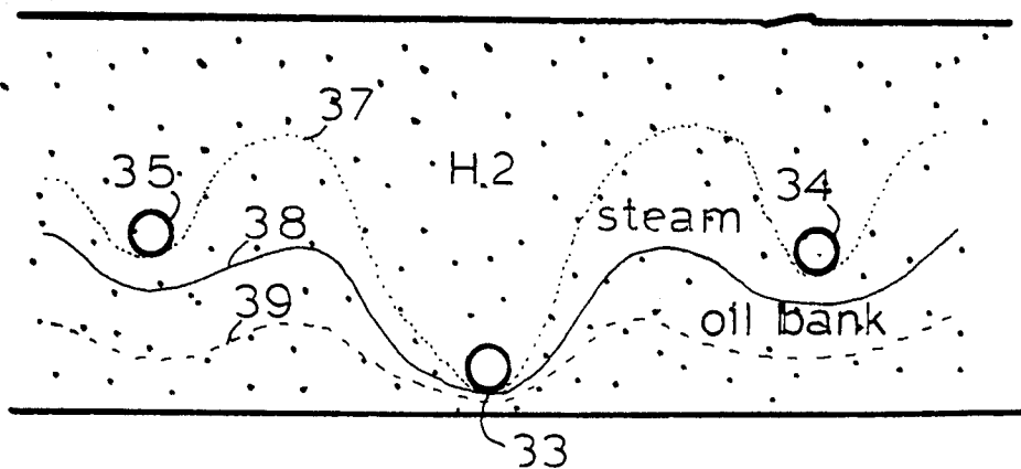
fig.11 SECTION BB
