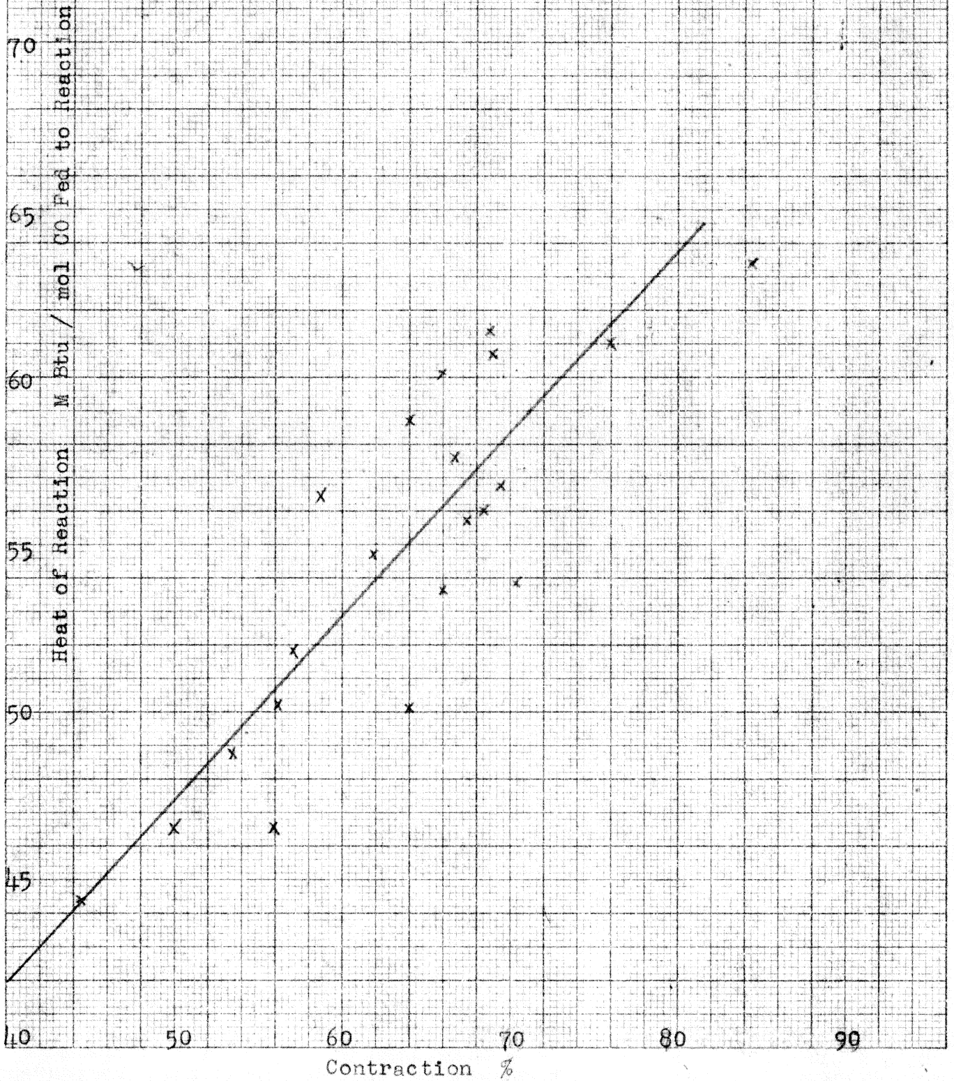
FIGURE III MONTEBELLO SYNTHESIS UNIT Heat of Reaction vs. % Contraction
