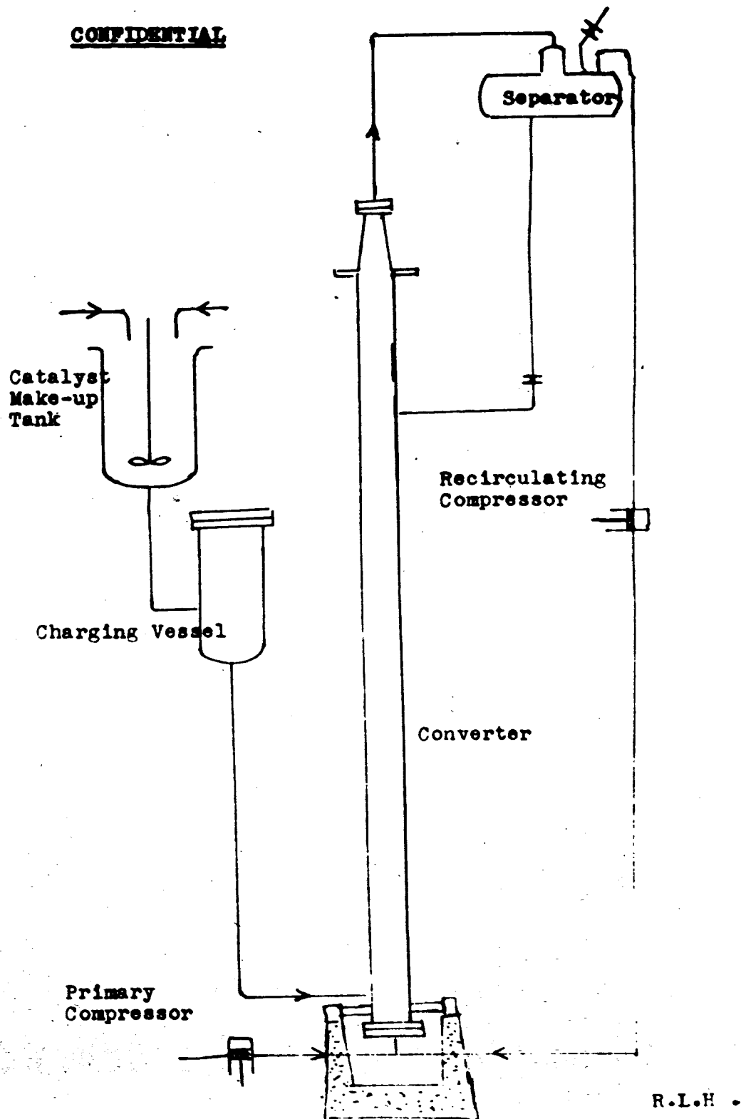
DIAGRAM OF CXO UNIT OBERHAUSEN-HOLDEN
