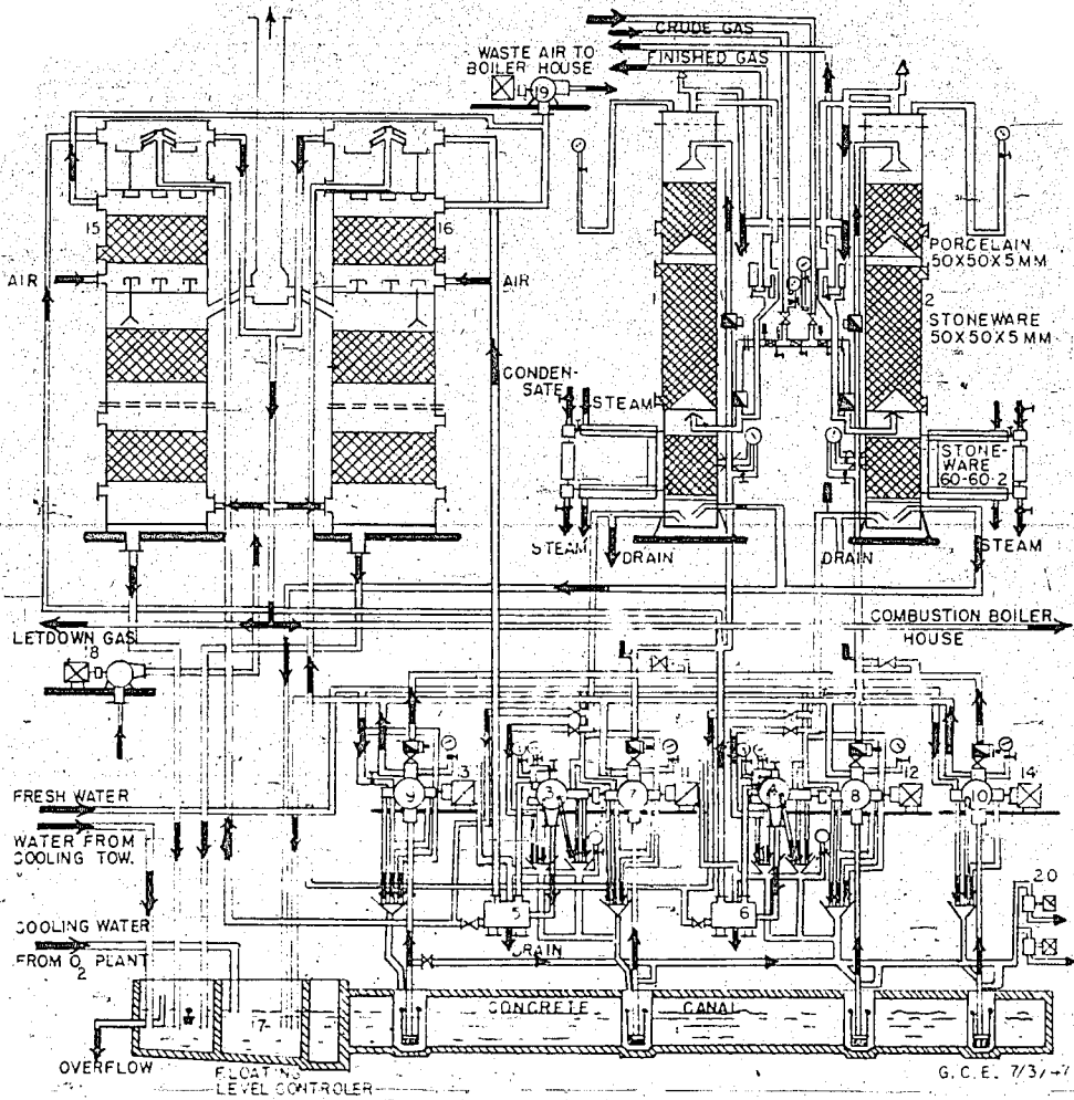
FLOW SHEET OF A PRESSURE WATER WASH PROCESS - ITEM 24
