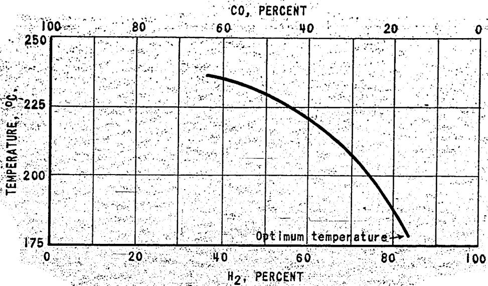
Figure 7. -- Variation in temperature with synthesis gas composition.
