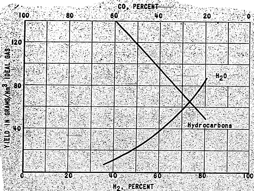
Figure 8. - Variation in yield with synthesis gas composition.
