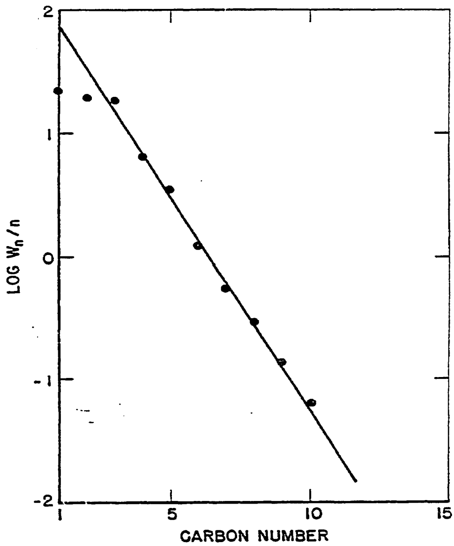
Figure 14 - Anderson - Schulz - Flory Plot for Fe-Mn Catalyst.
