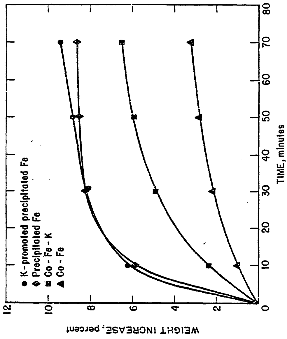
Figure 8 - Carbiding of Iron Catalysts with 1/1 Syn Gas at 493°K.
