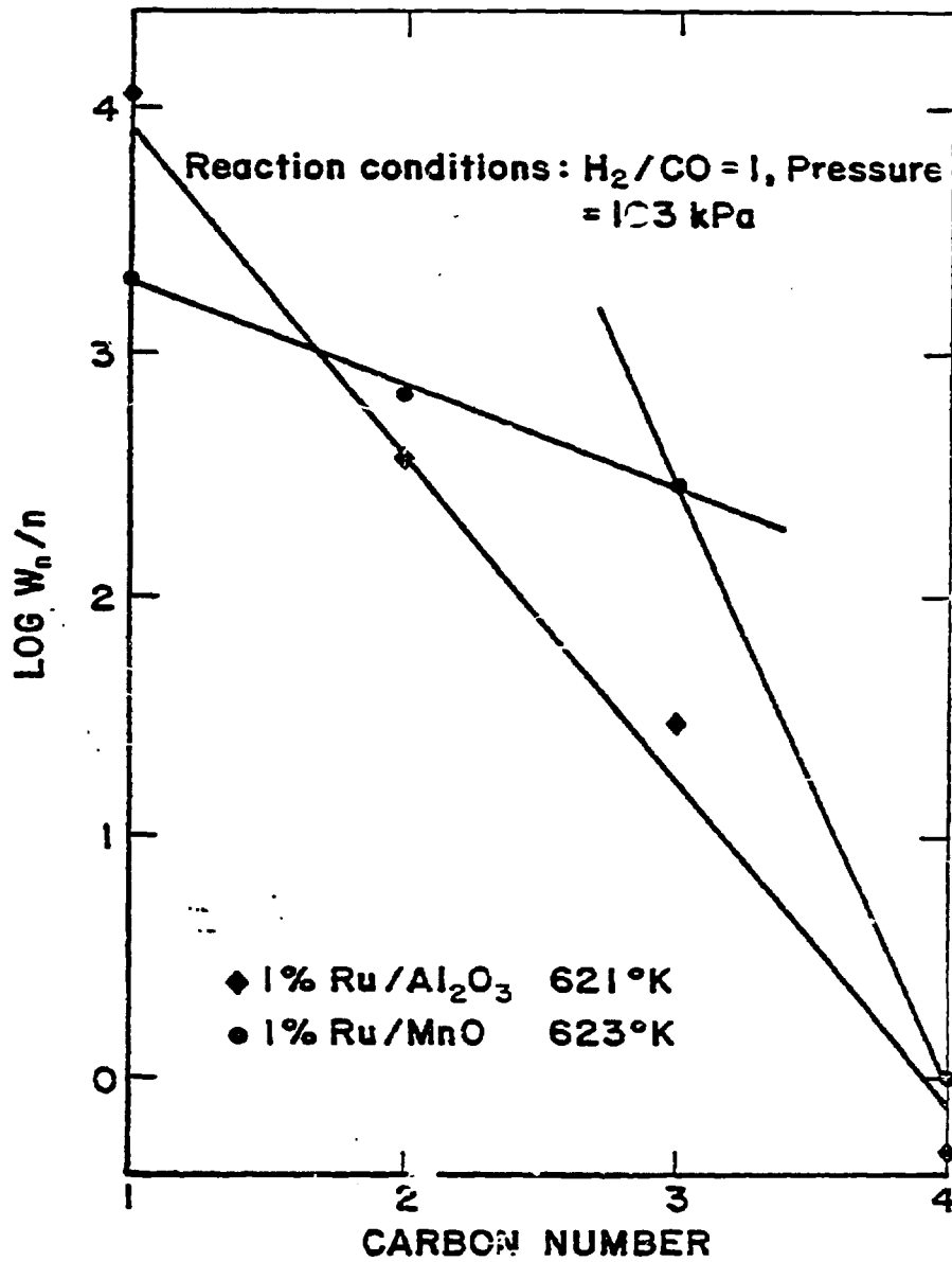
Figure 15 - Anderson - Schulz - Flory Plot for Ru Catalysis .
