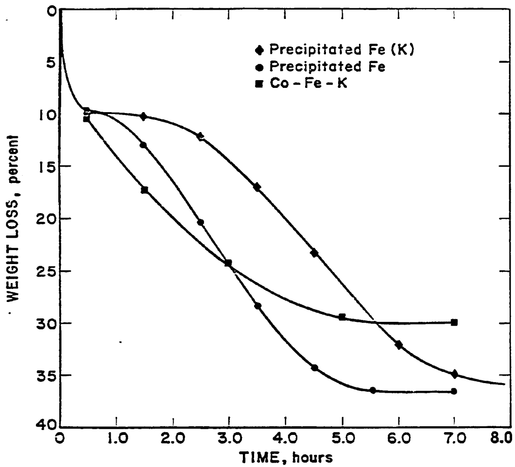
Figure 7 - Reduction of Precipitated Iron Catalysts in H 2 at 523° K.
