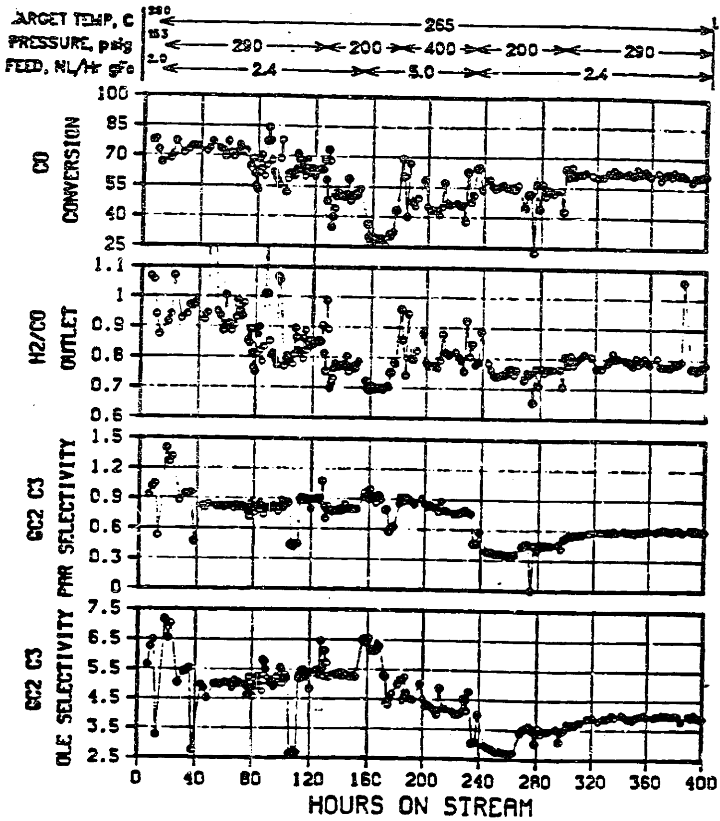
FIGURE A-40 SUMMARY DATA FOR UCI-"START-UP" CATALYST - RUN 53
