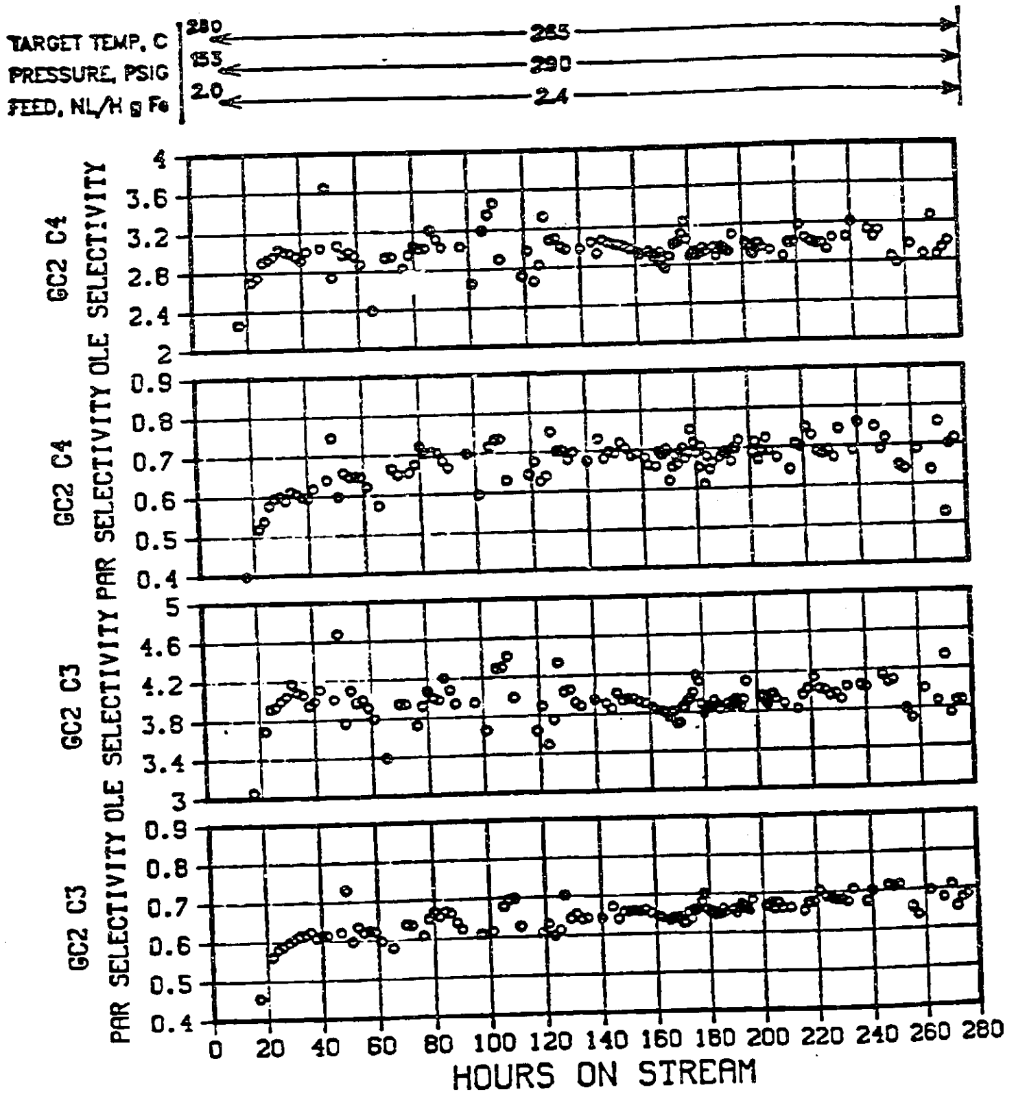
FIGURE A-29 SUMMARY DATA FOR UCI-"A" CATALYST - RUN 59
