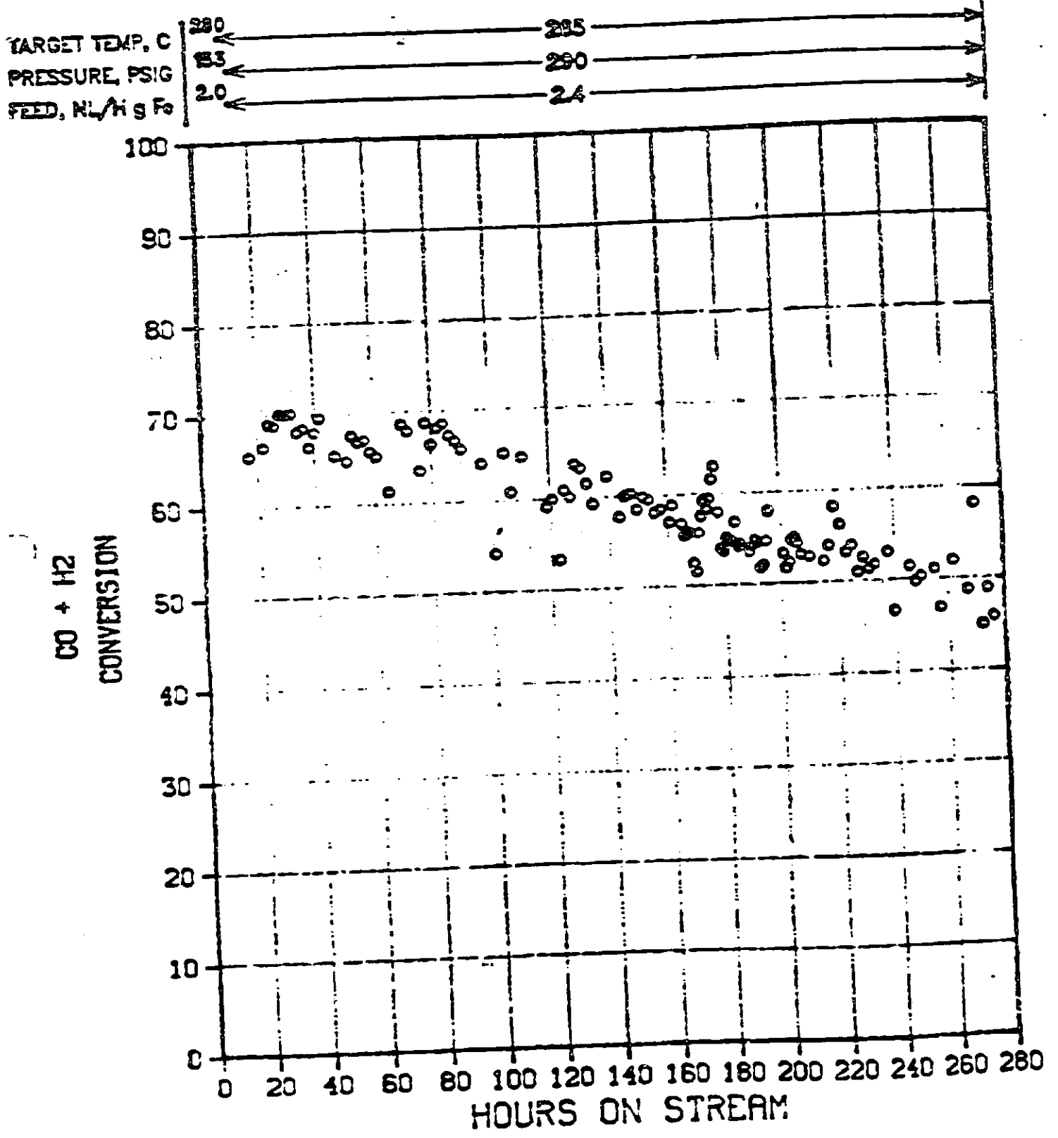
FIGURE A-23 SUMMARY DATA FOR UCI-"A" CATALYST - RUN 50
