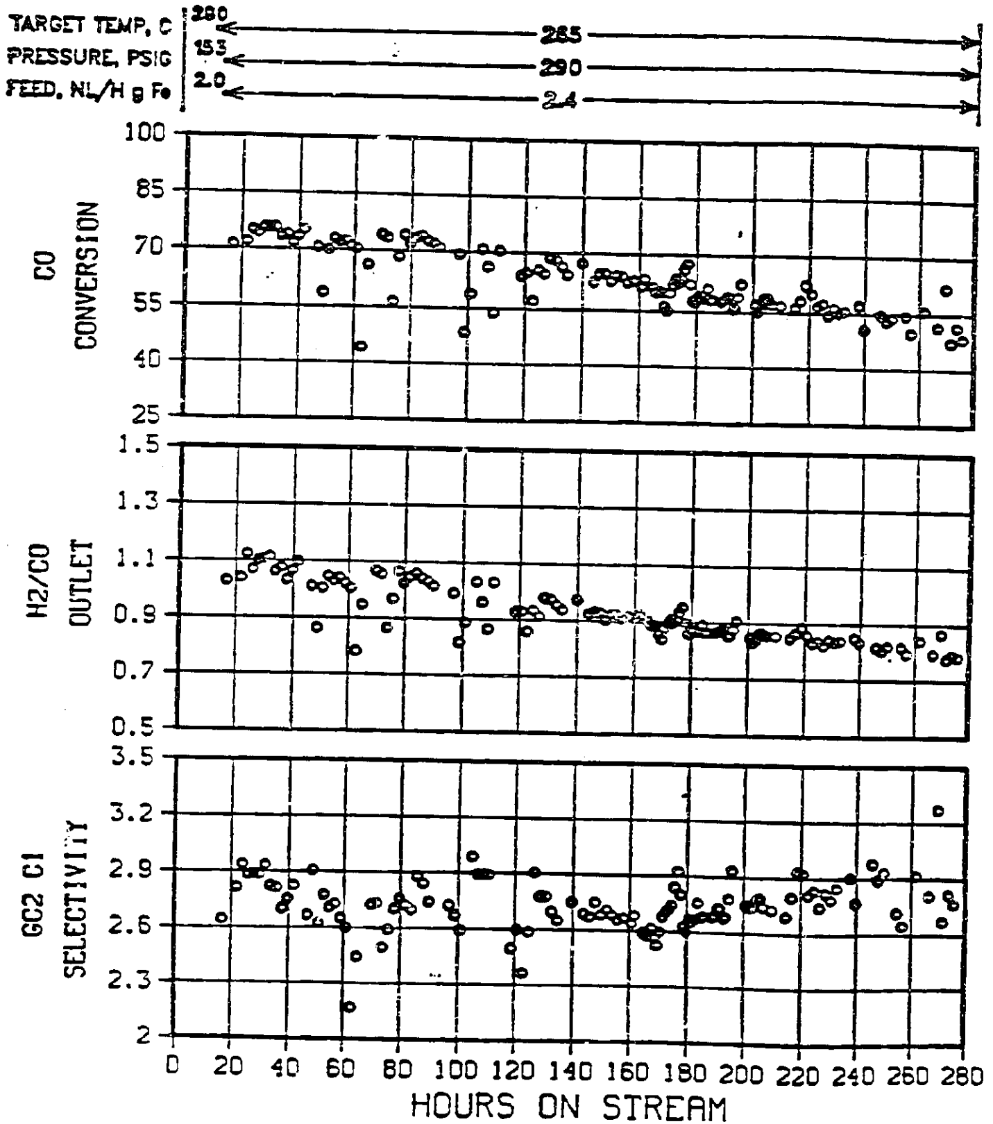
FIGURE A-26 SUMMARY DATA FOR UCI-"A" CATALYST - RUN 50
