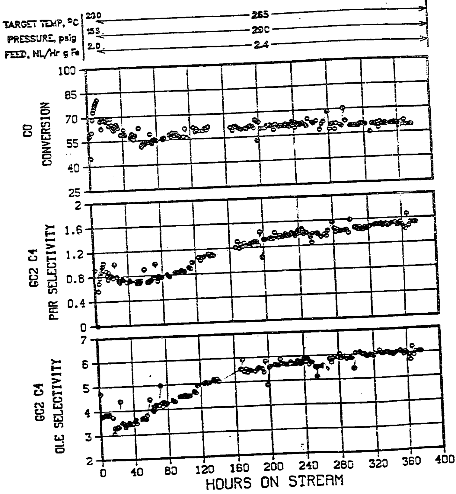
FIGURE A-35 SUMMARY DATA FOR UCI-"B" CATALYST - RUN 51
