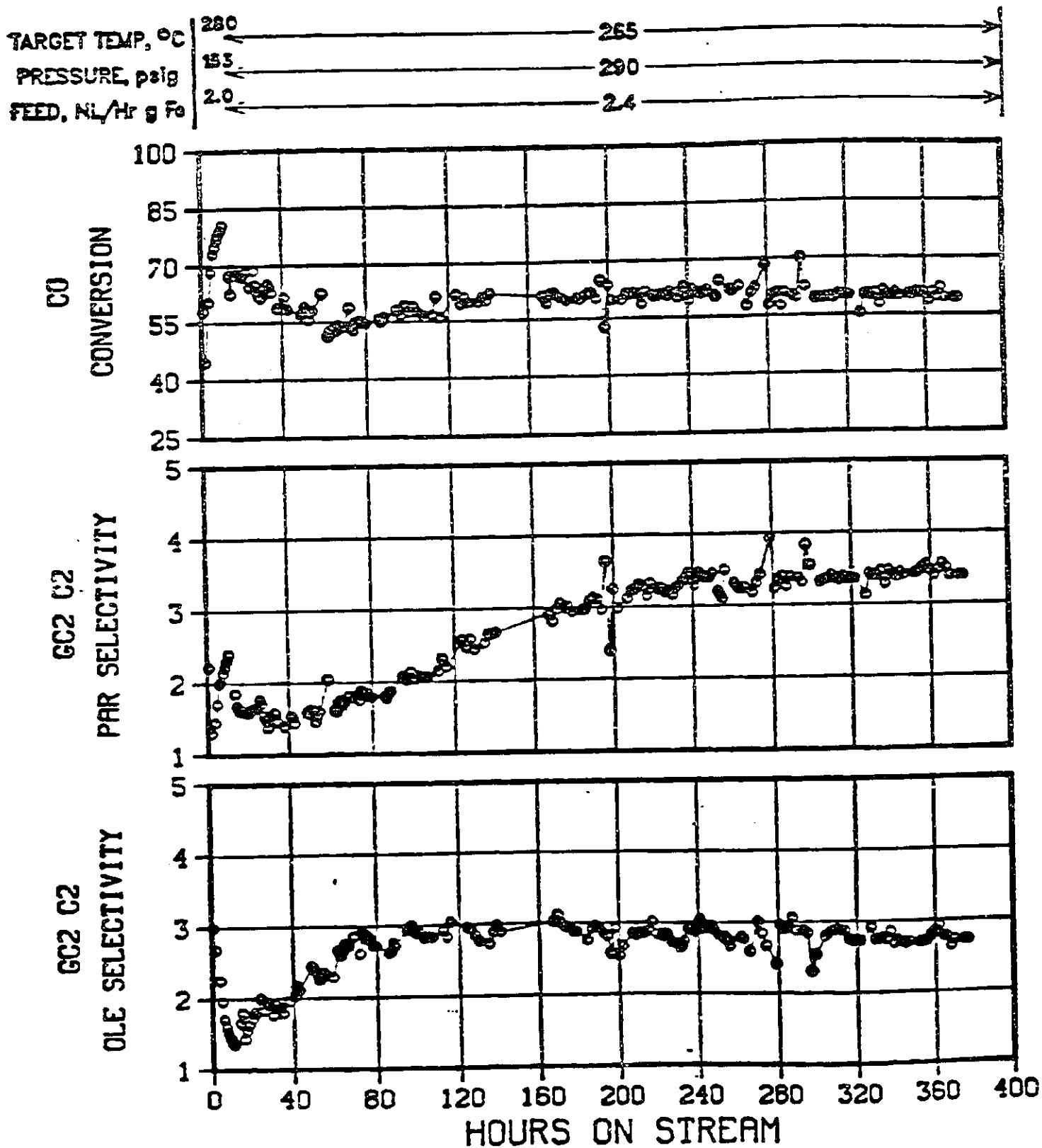
FIGURE A-33 SUMMARY DATA FOR UCI-"B" CATALYST - RUN 51
