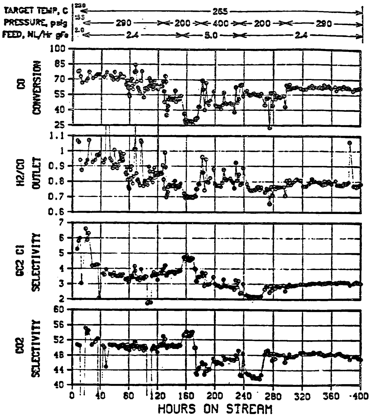
FIGURE A-38 SUMMARY DATA FOR UCI-"START-UP" CATALYST - RUN 53
