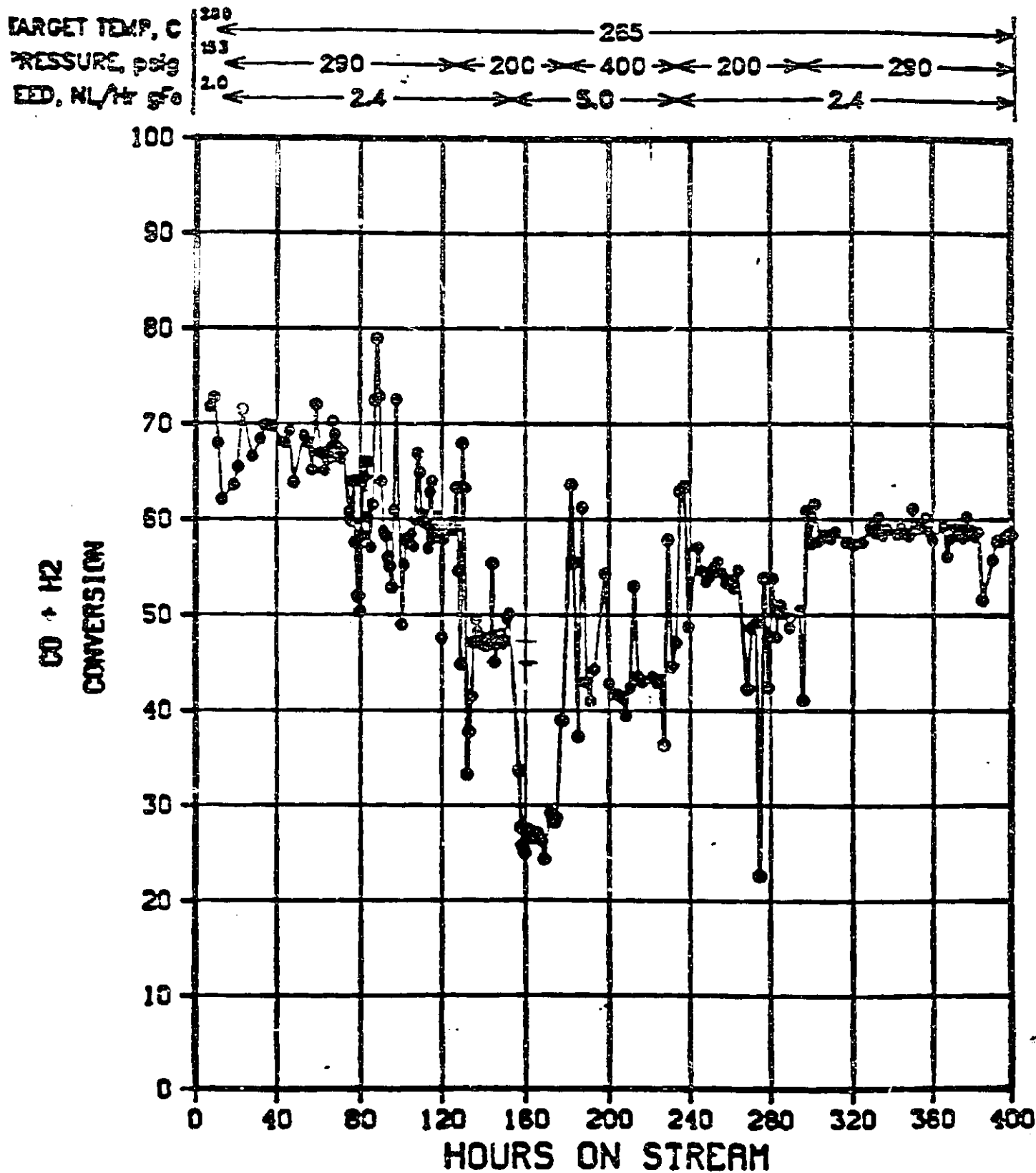
FIGURE A-36 SUMMARY DATA FOR UCI-"START-UP" CATALYST - RUN 53
