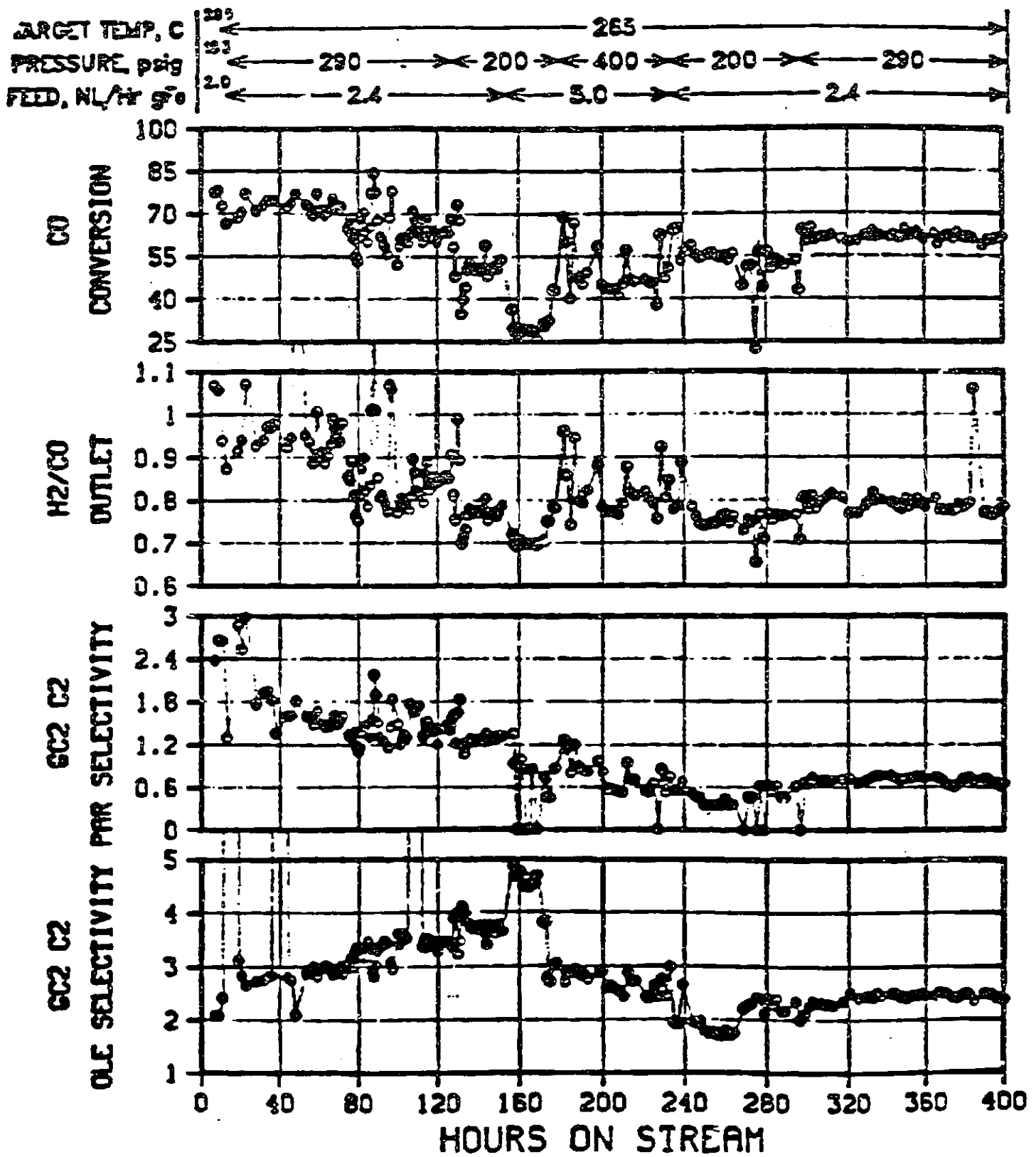
FIGURE A-39 SUMMARY DATA FOR UCI-"START-UP" CATALYST - RUN 53
