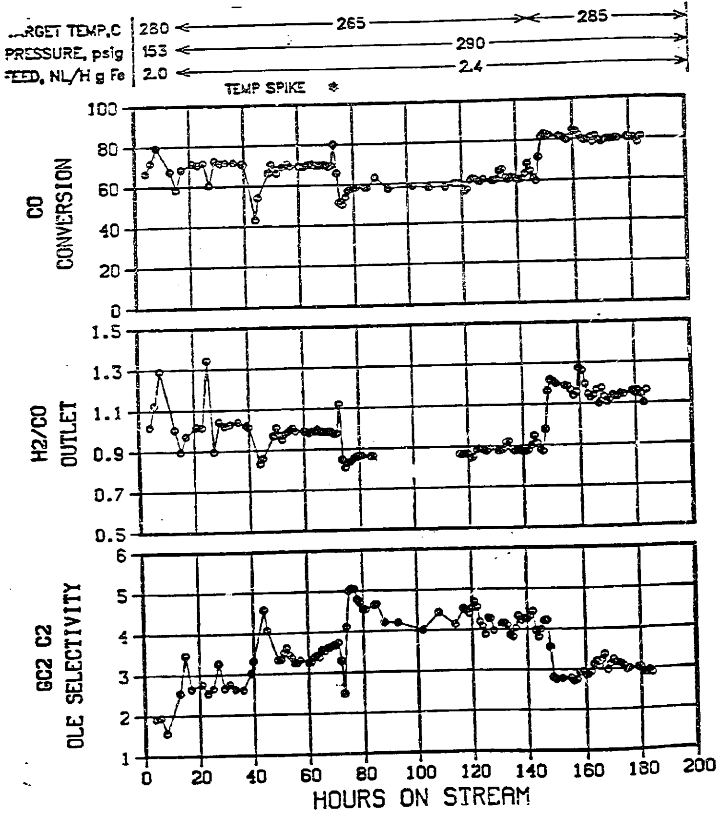
FIGURE A-21 SUMMARY DATA FOR UCI-"O" CATALYST - RUN 48
