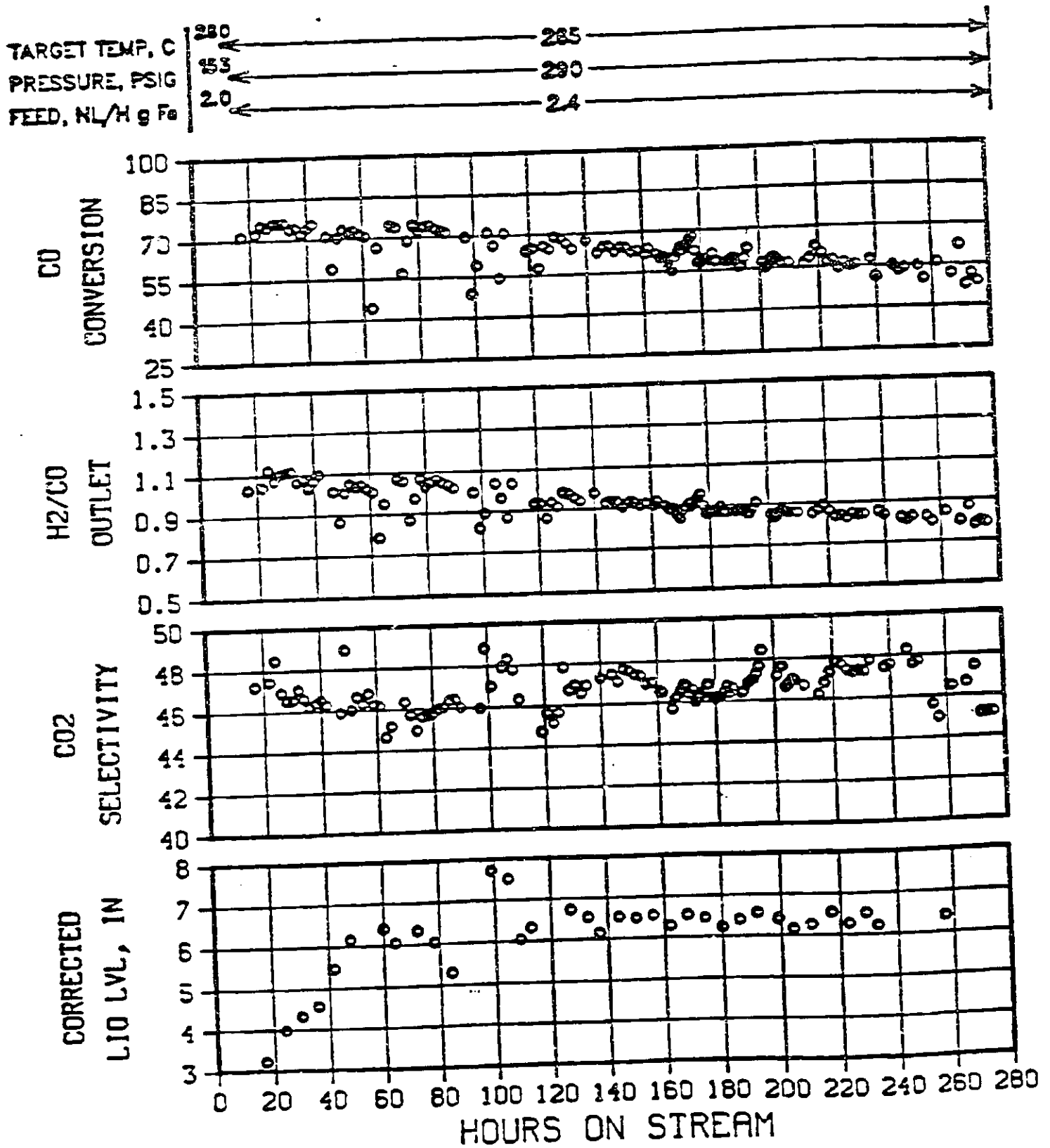
FIGURE A-25 SUMMARY DATA FOR UCI-"A" CATALYST - RUN 50
