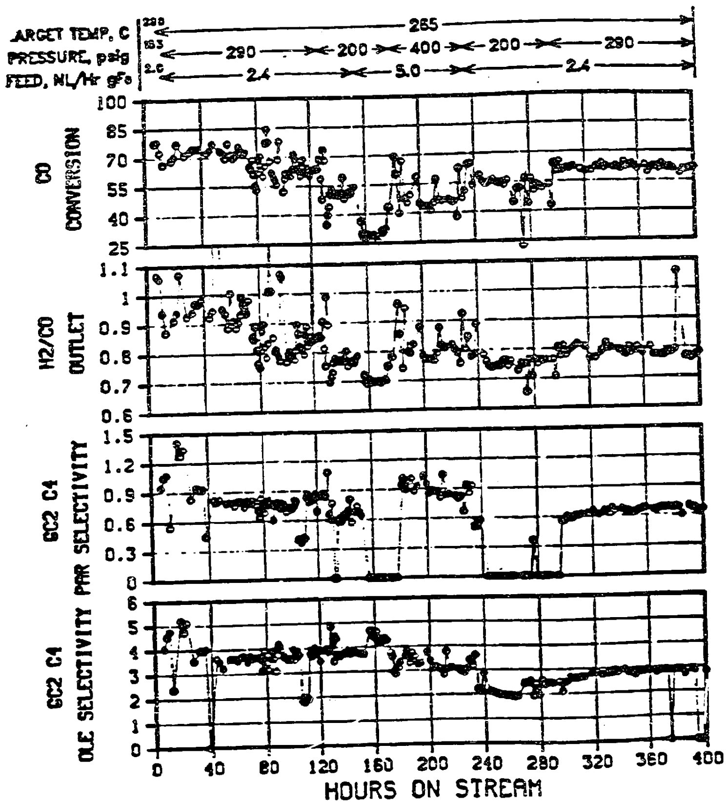
FIGURE A-41 SUMMARY DATA FOR UCI-"START-UP" CATALYST - RUN 53
