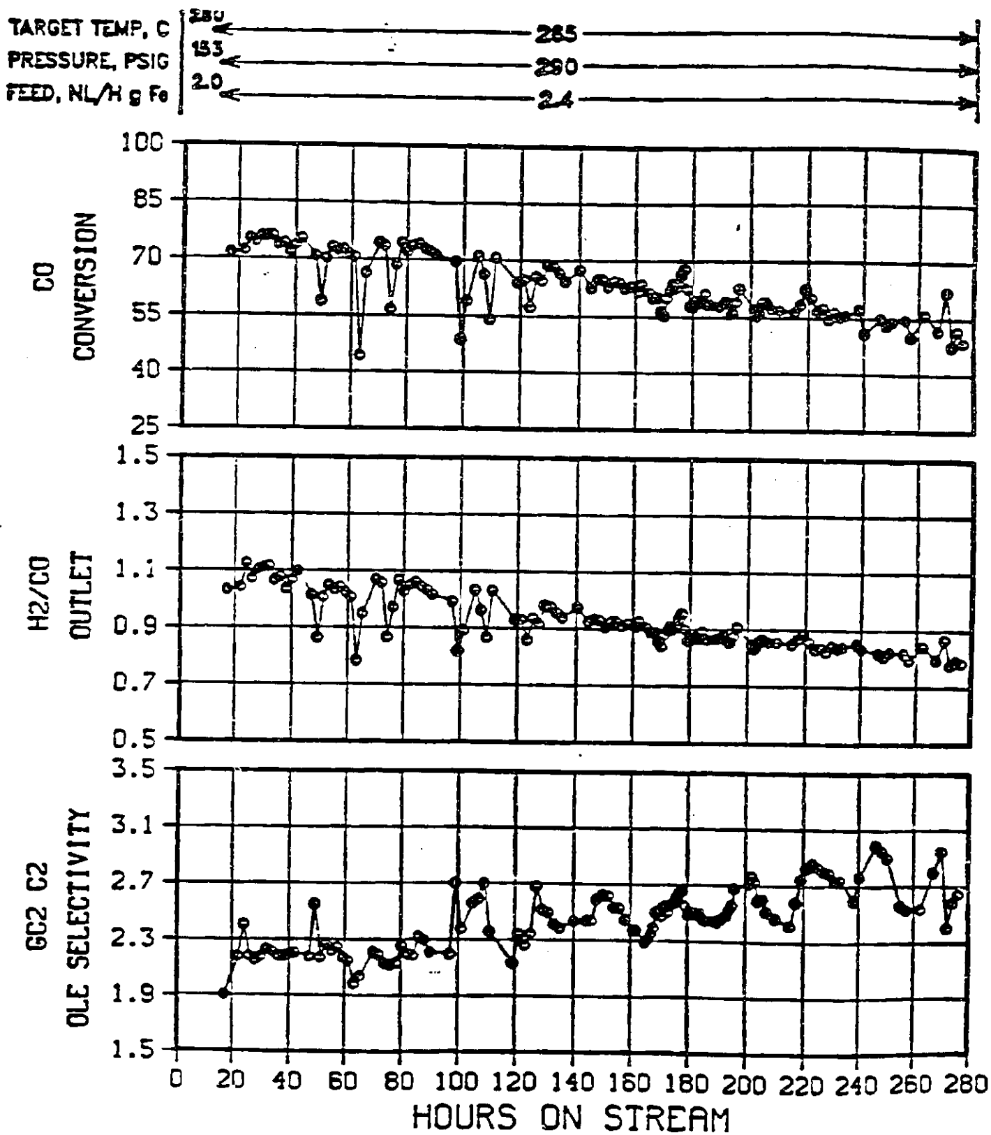
FIGURE A-28 SUMMARY DATA FOR UCI-"A" CATALYST - RUN 50
