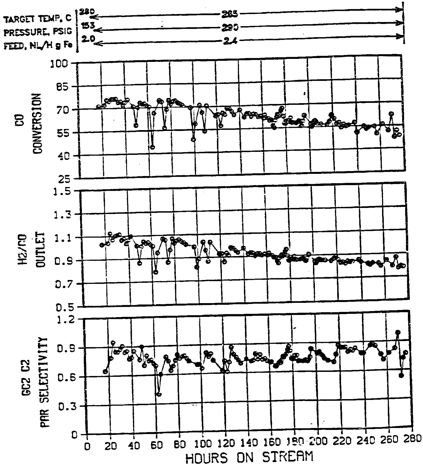
FIGURE A-27 SUMMARY DATA FOR UCI-"A" CATALYST - RUN 50
