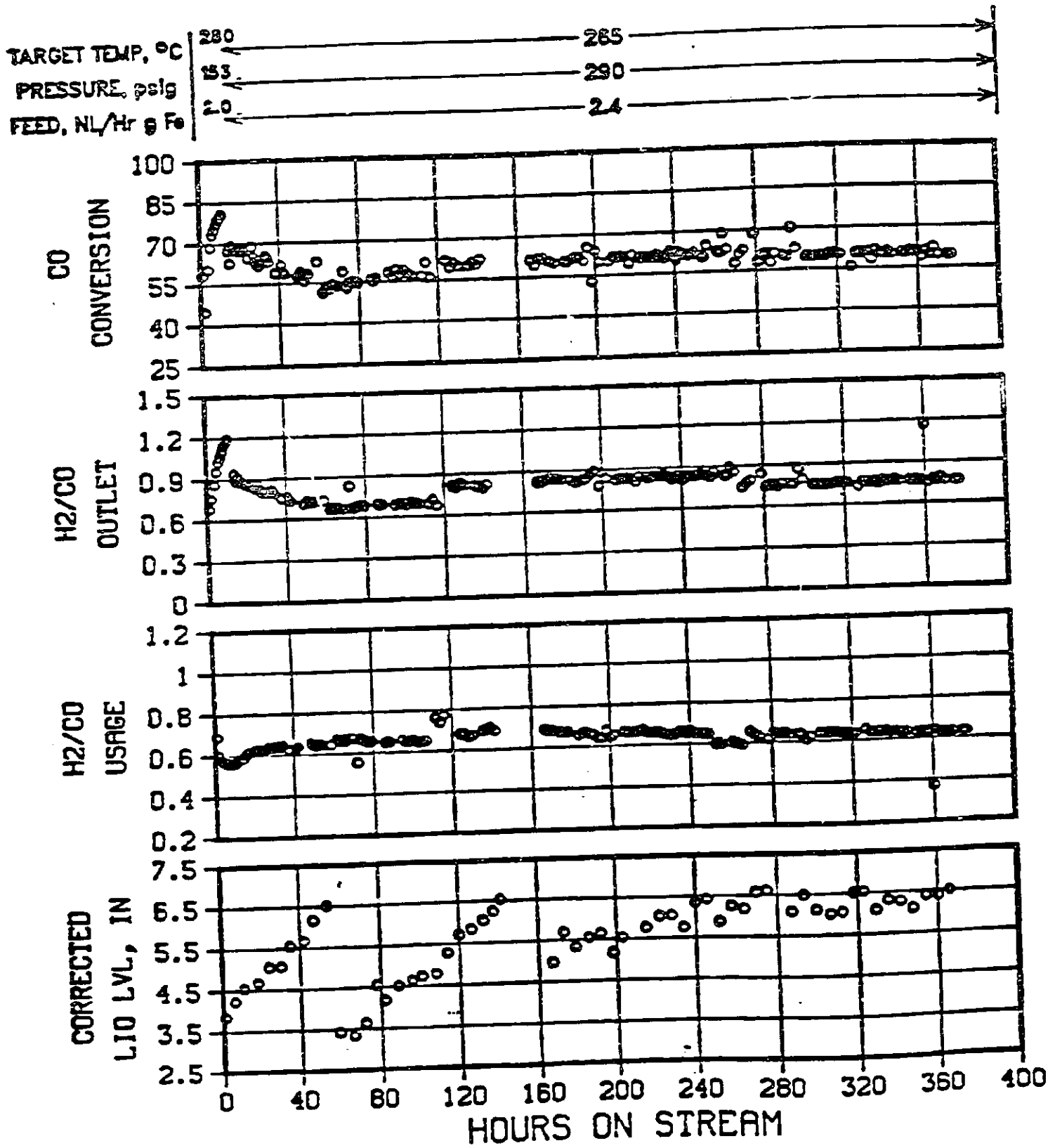
FIGURE A-31 SUMMARY DATA FOR UCI-"B" CATALYST - RUN 51
