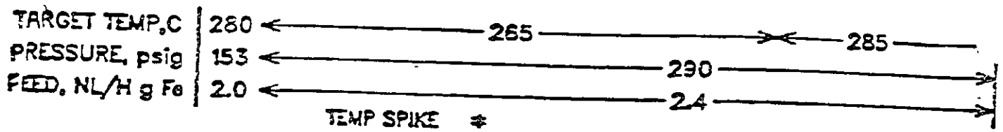
FIGURE A-18 SUMMARY DATA FOR UCI-"O" CATALYST - RUN 48
