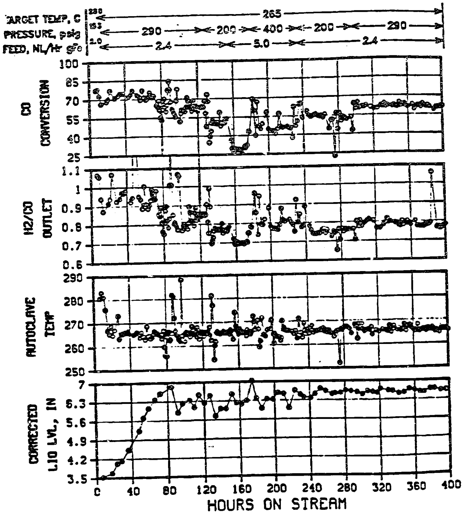
FIGURE A-37 SUMMARY DATA FOR UCI-"START-UP" CATALYST - RUN 53
