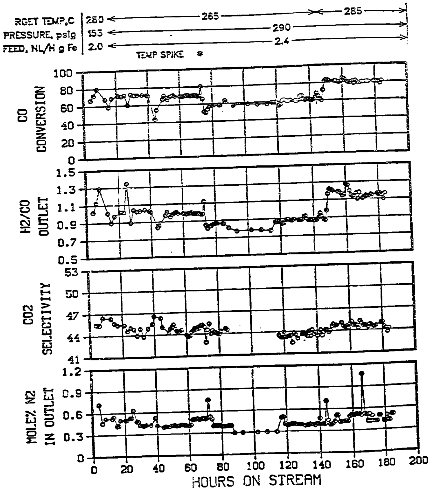
FIGURE A-17 SUMMARY DATA FOR UCI-"O" CATALYST - RUN 48
