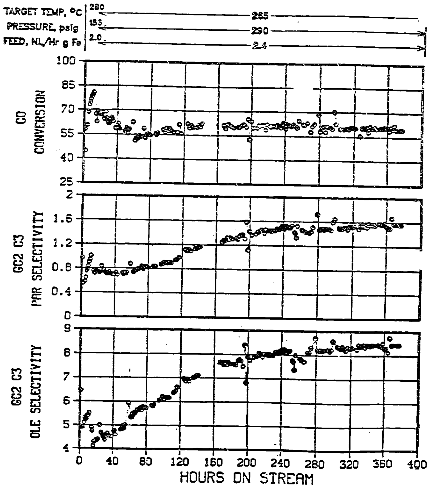
FIGURE A-34 SUMMARY DATA FOR UCI-"B" CATALYST - RUN 51
