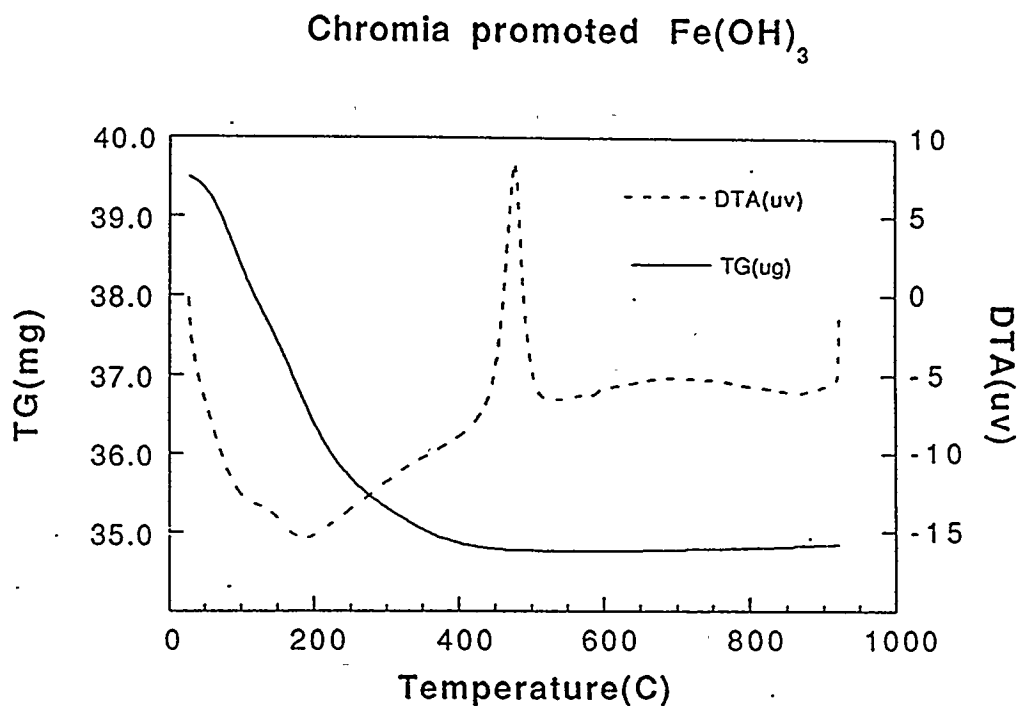
Figure IV.7.2. Thermal gravimetric (TG) and differential thermal analysis (DTA) curves for the 6% chromium oxide promoted iron oxide.
