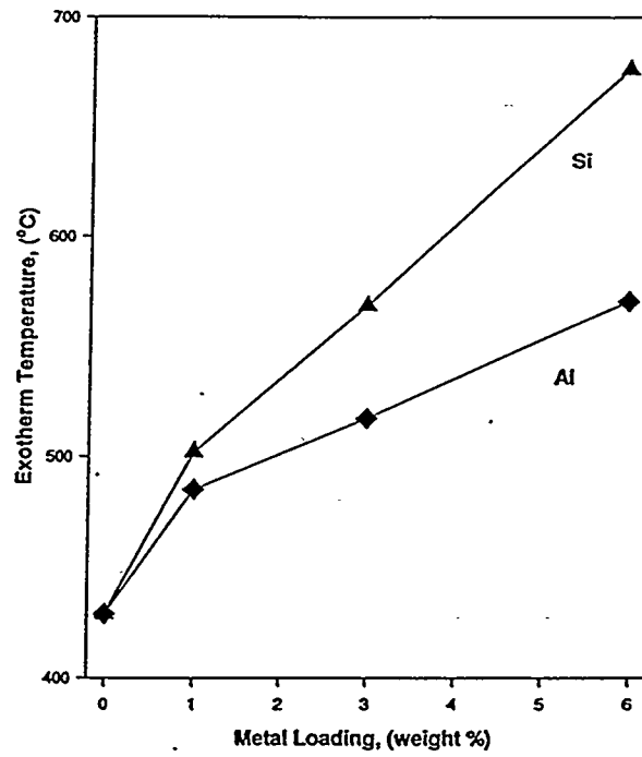
Figure IV.7.5. Exotherm temperature for Si and Al promoted iron oxides.
