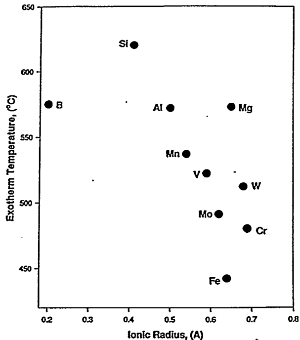
Figure IV.7.4. Exotherm temperature for 6% metal oxide promoted and unpromoted iron oxides.
