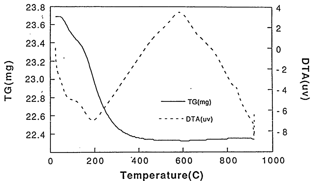
Figure IV.7.3. Thermal gravimetric (TG) and differential thermal analysis (DTA) curves for the 6% barium oxide promoted iron oxide.
