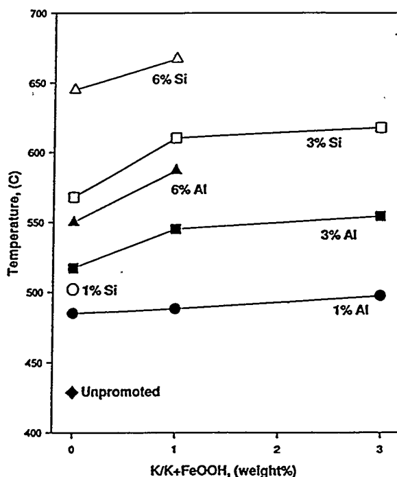
Figure IV.7.7. Exotherm temperature for K and Si or Al doubly promoted iron oxides.
