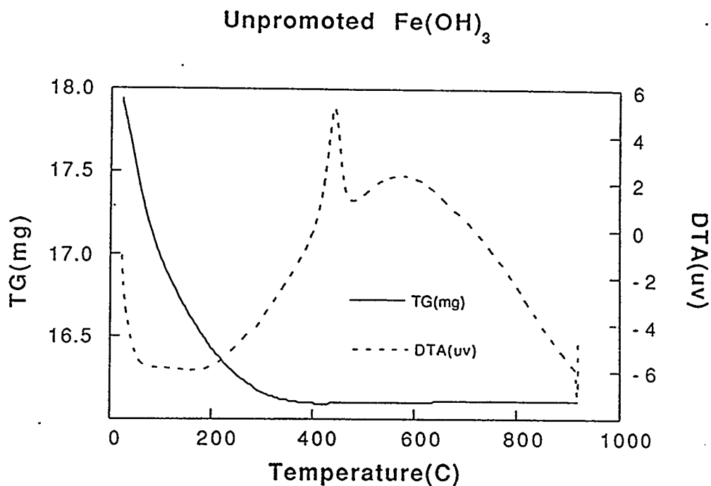
Figure IV.7.1. Thermal gravimetric (TG) and differential thermal analysis (DTA) curves for the unpromoted iron oxide sample.
