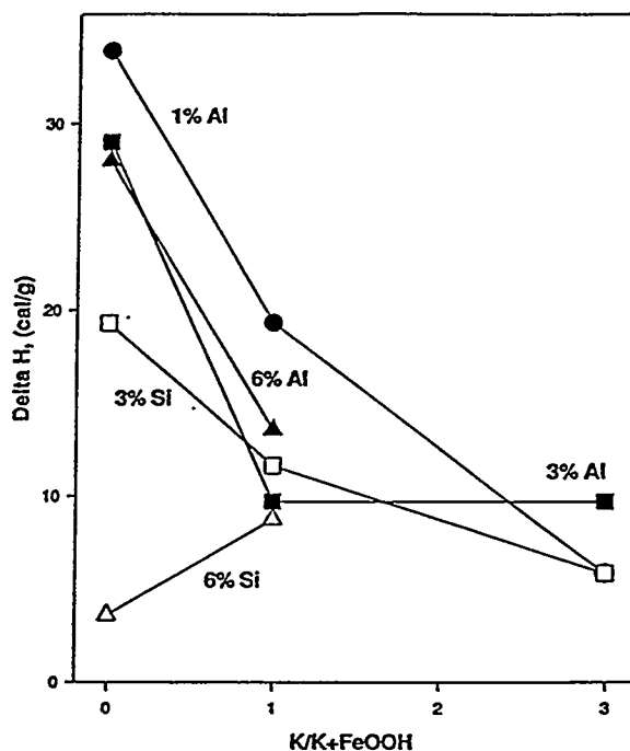
Figure IV.7.8. Heat liberated during the exothermic event for K and Si or Al doubly promoted iron oxides.
