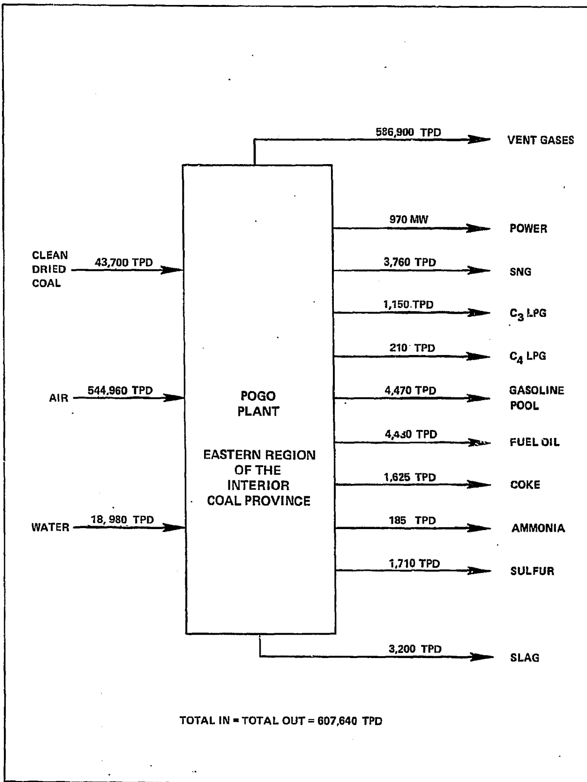
Figure 8-1 - Overall Material Balance — Process and Power Units
