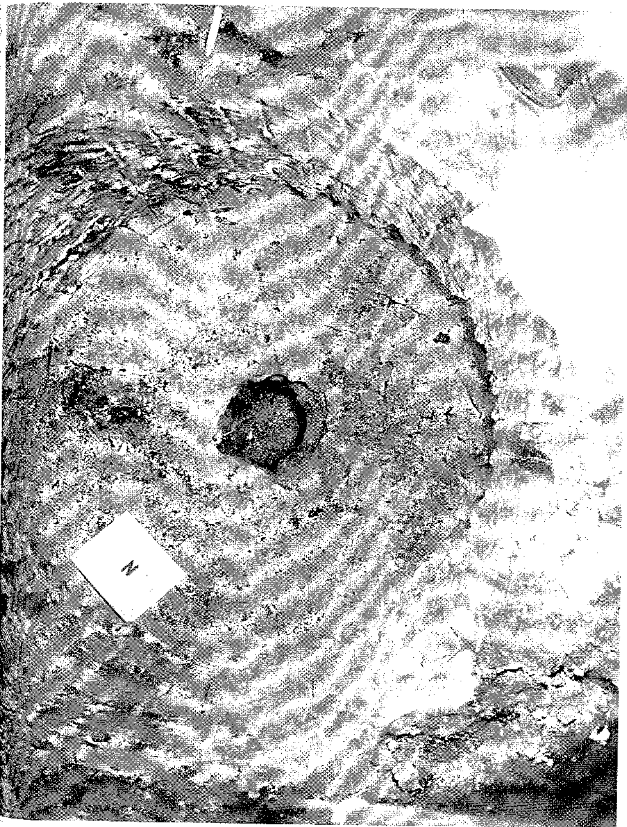
Figure 16. - Slag tap and primary zone after run 34.
