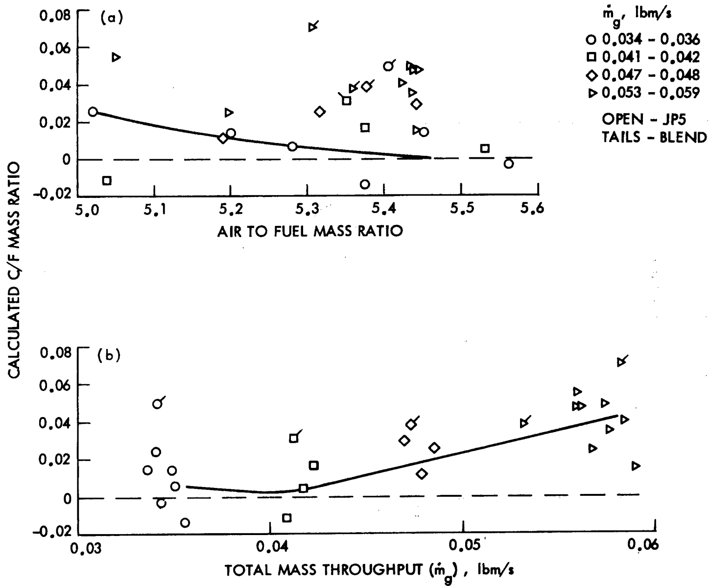
Figure 17. Calculated Solid Carbon Production for Generator L: (a) Versus Air to Fuel Ratio; (b) Versus Mass Throughput
