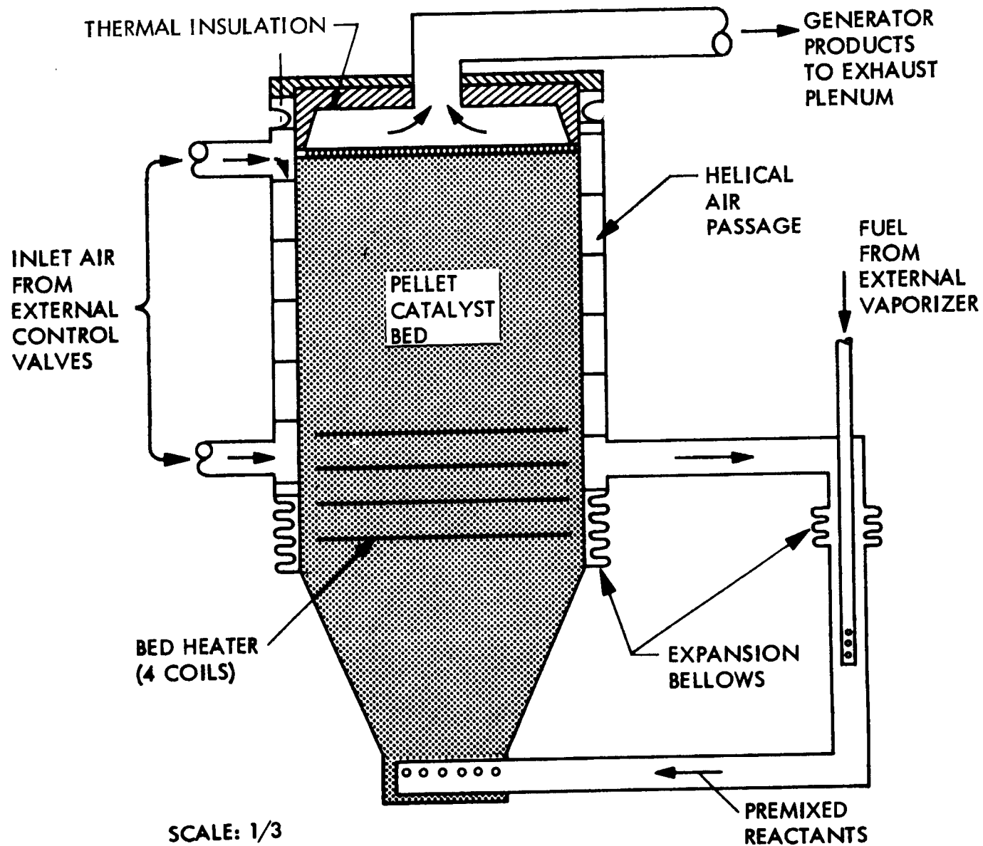
Figure 9. Schematic of Generator L
