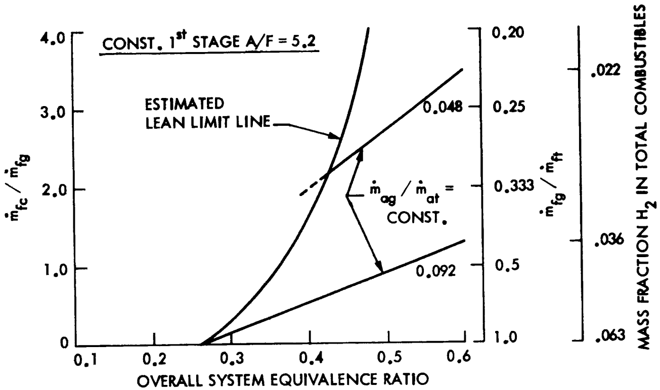
Figure 6. Conceptual Operating Map for 2-Stage Combustion System
