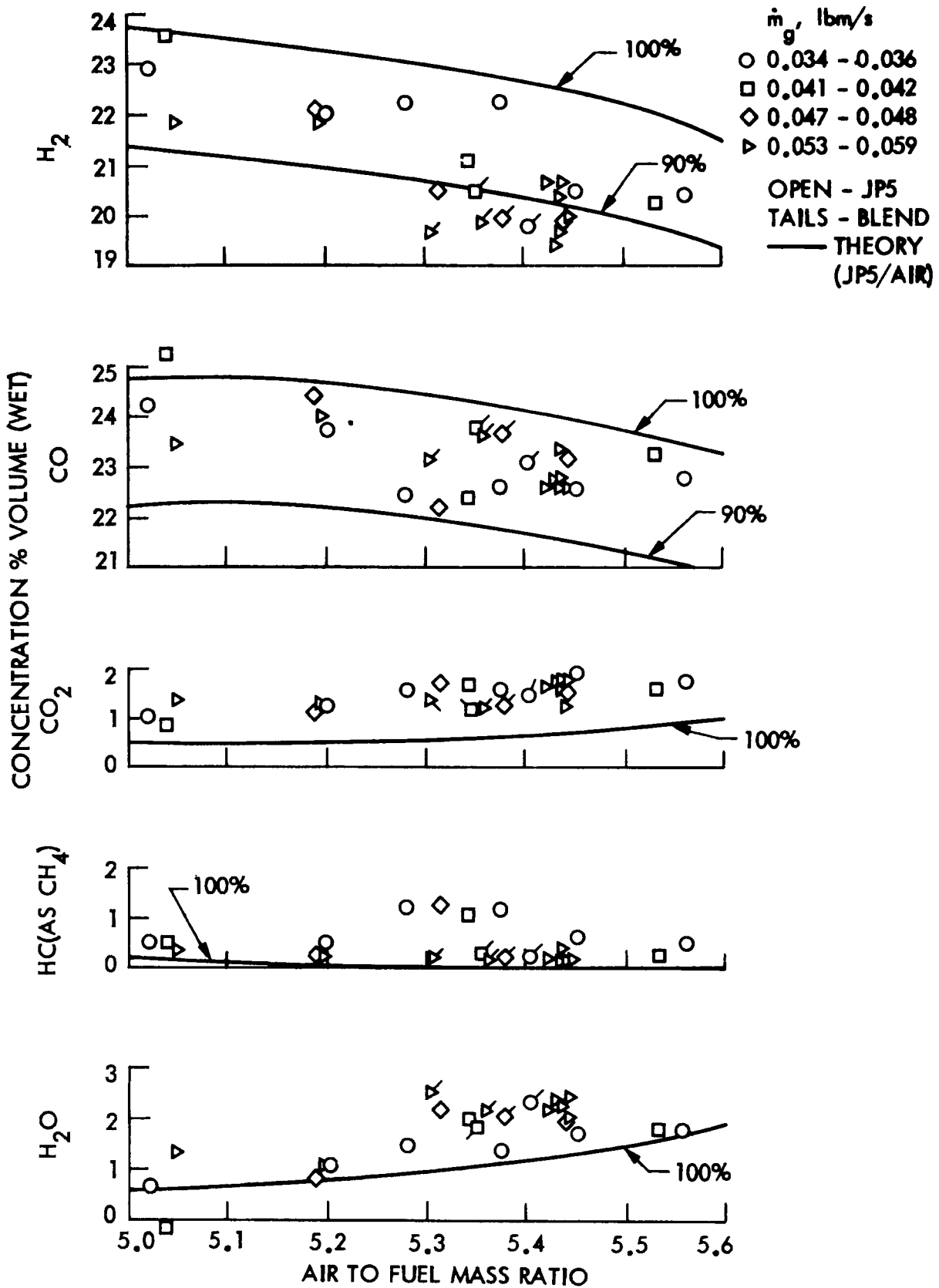
Figure 13. Product Compositions for Generator L
