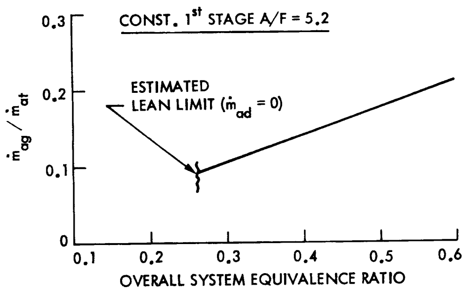
Figure 7. Variation of Air Split for All Fuel Through 1 st Stage
