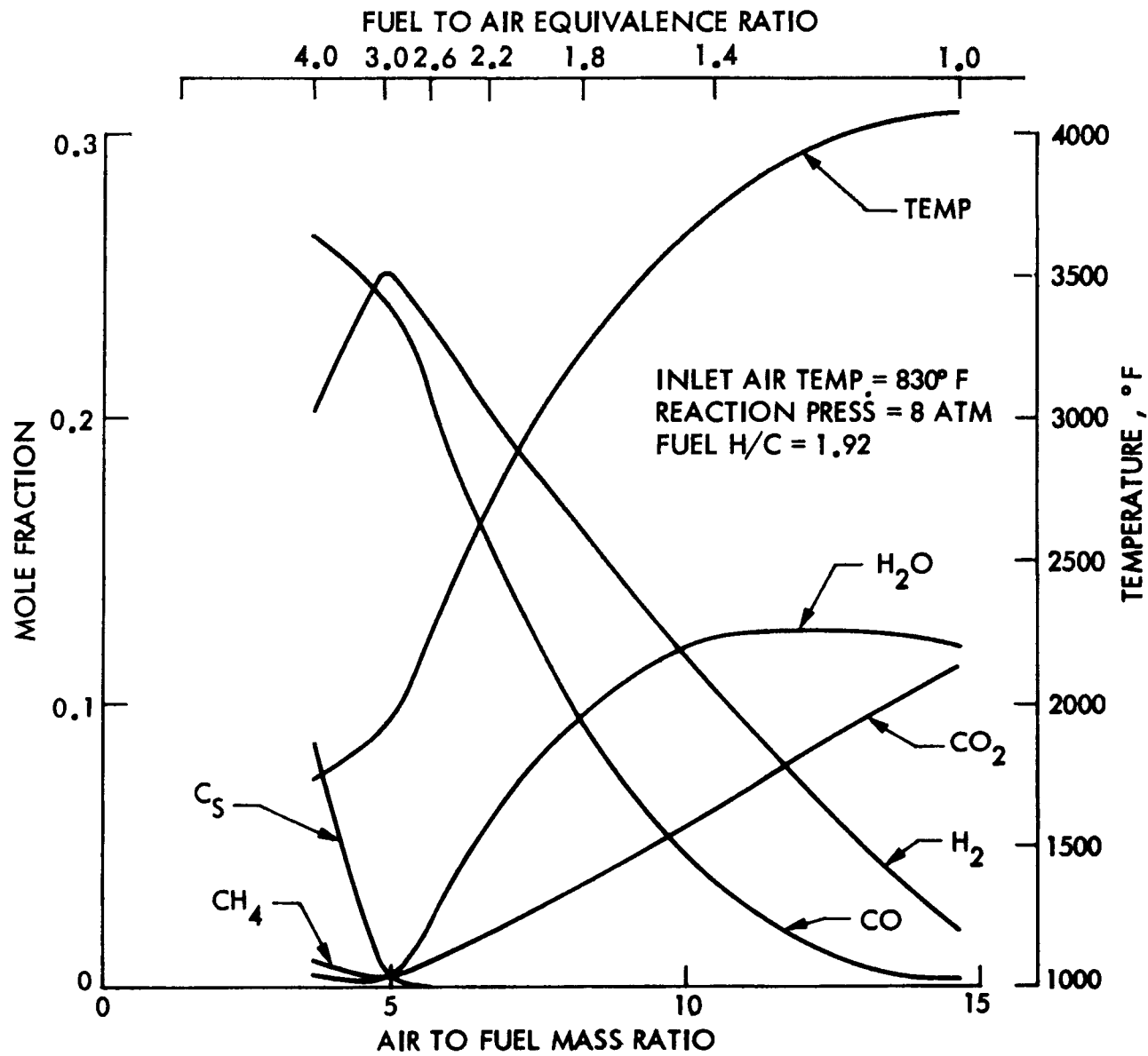
Figure 2. Theoretical Equilibrium Composition and Temperature - Cruise Condition
