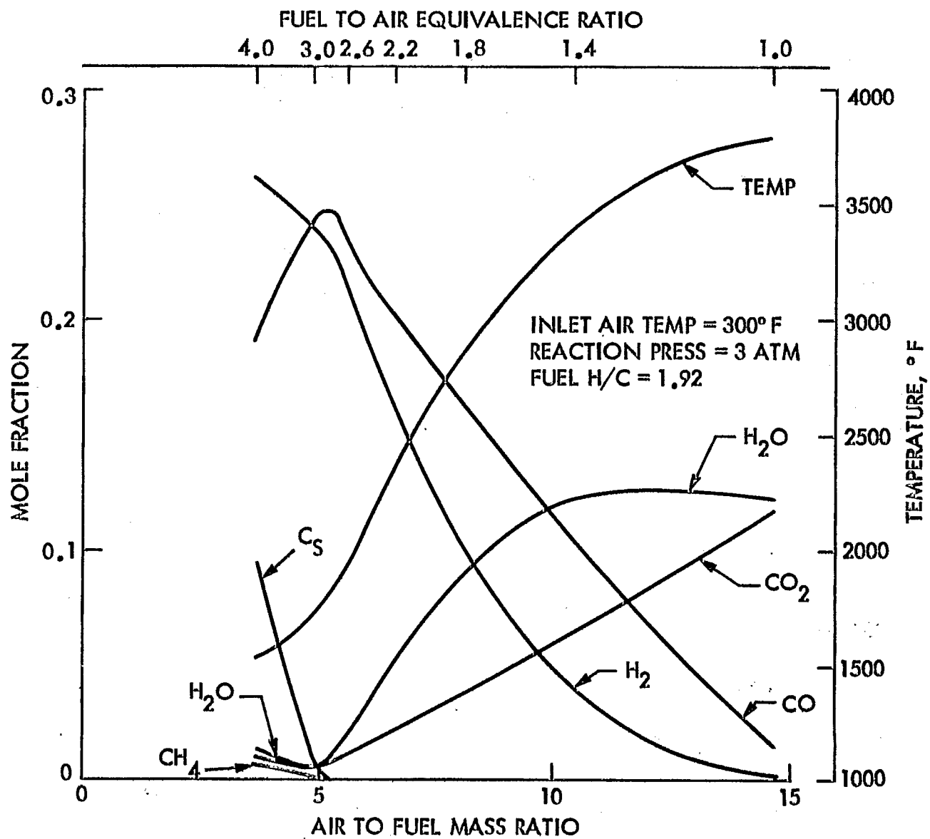
Figure 1. Theoretical Equilibrium Composition and Temperature - Idle Condition
