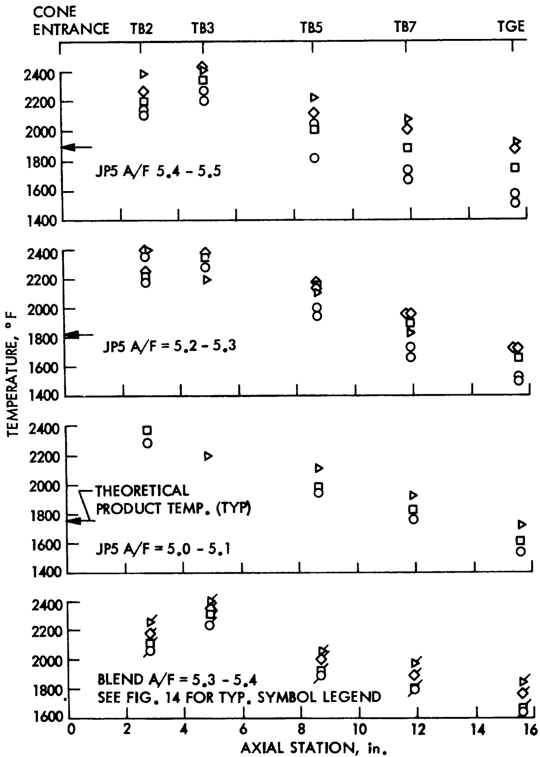
Figure 15. Axial Profiles of Bed Temperature for Generator L
