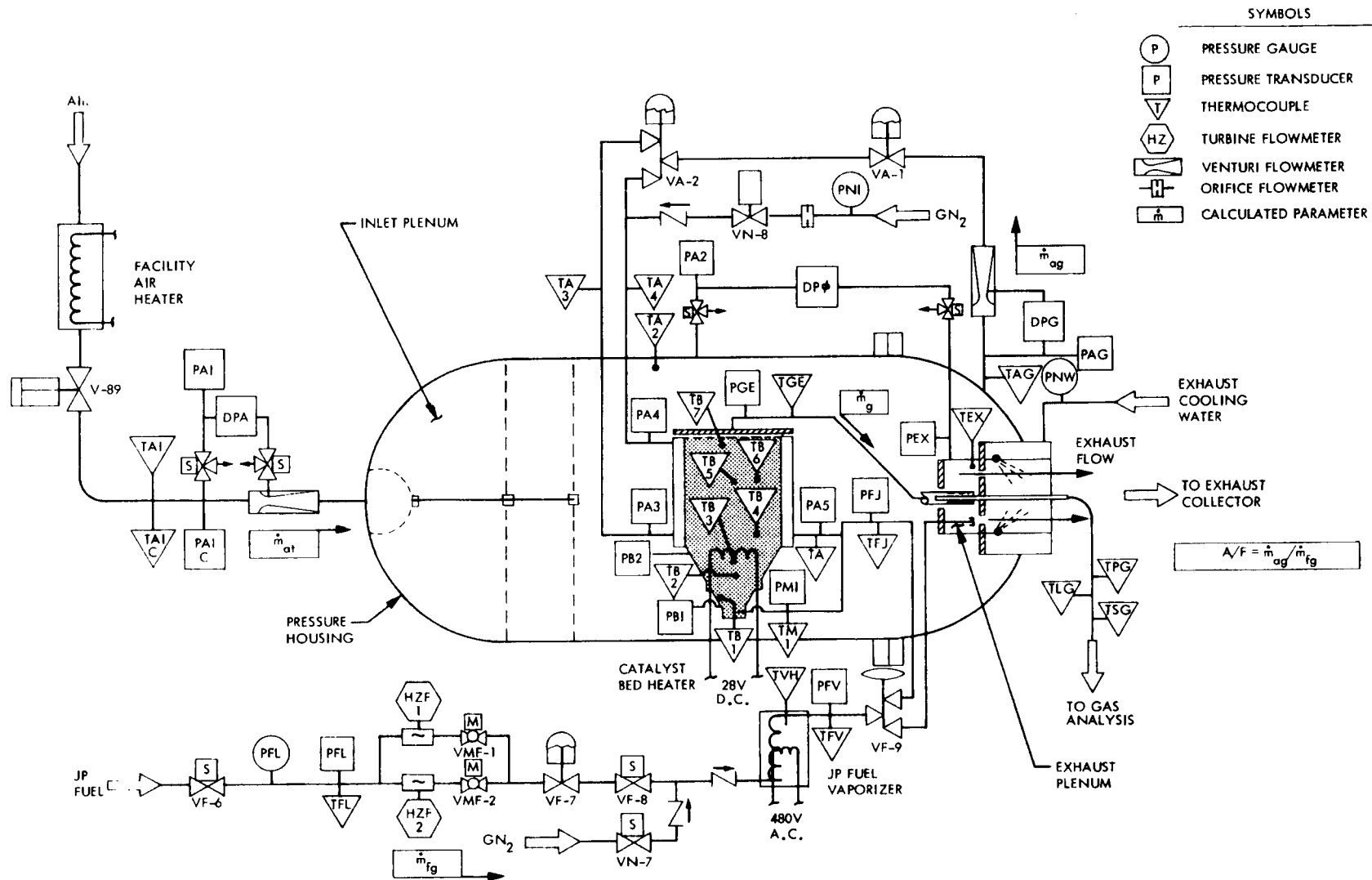
Figure 11. Schematic of Generator L Test Setup in High Pressure Combustion Facility
