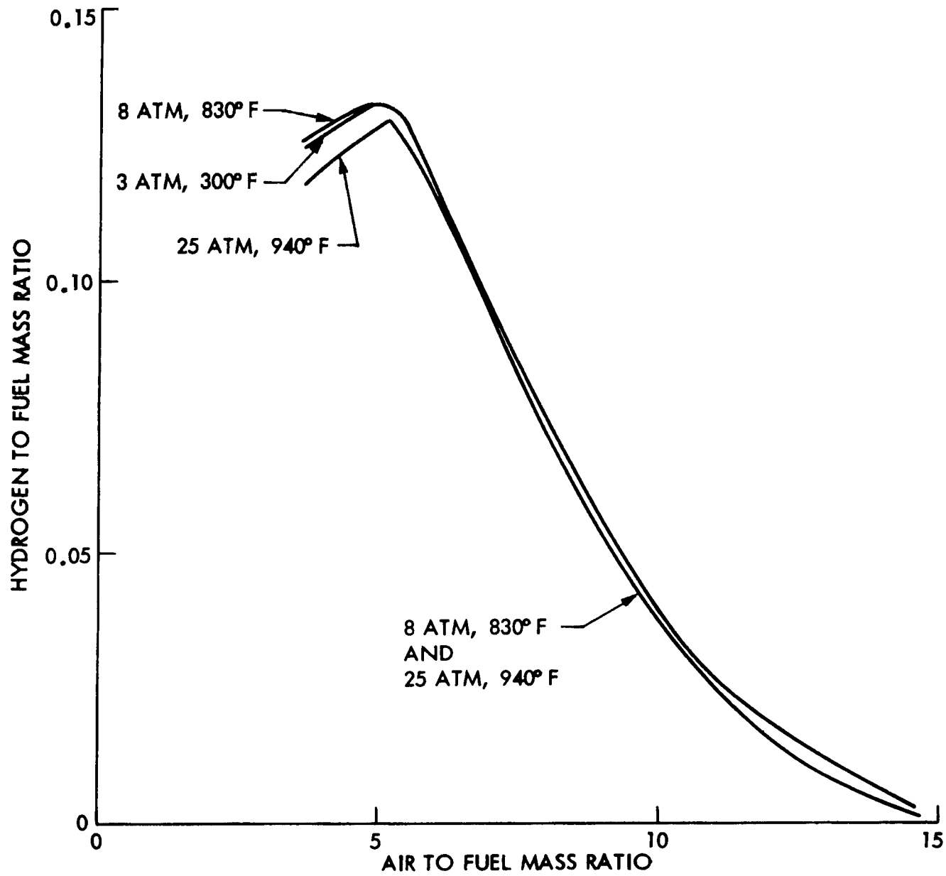
Figure 4. Theoretical Hydrogen to Fuel Mass Ratio for Various Power Conditions
