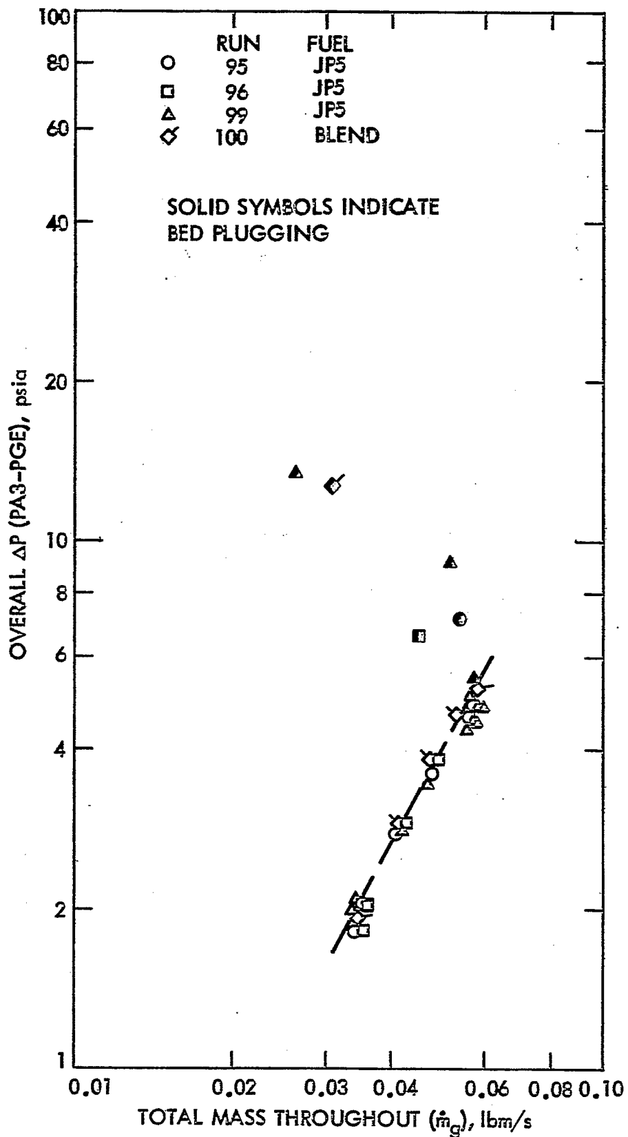
Figure 16. Overall Pressure Drop Characteristics For Generator L During Operation
