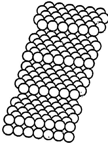
fcc (100)
