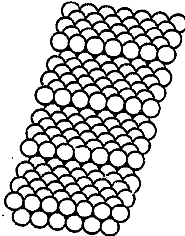
fcc (210)
