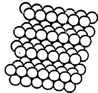
fcc (211)
