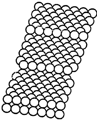
fcc (111)
