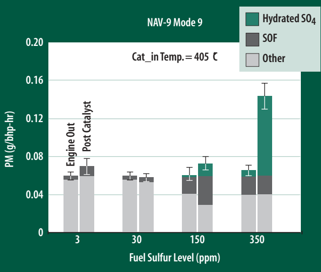
Figure 3. Engine-out and post-lean-NO x catalyst (fresh) emissions of PM and components under low-temperature (Navistar) applications using a Nav-9 mode 9 test (with 95% confidence intervals on estimated PM)
