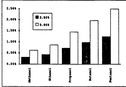
Fig. 2 The change in specific gravity of C 1 -C 5 alcohol-gasoline blends relative to neat gasoline.
