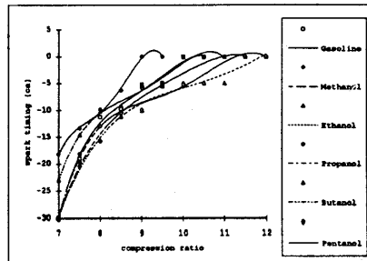
Fig. 10 Knock limiting spark timing at different compression ratios for blends with 2.5% oxygen content.
