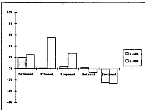
Fig.13 Comparison of alcohol-gasoline blends (2.5% and 5% oxygen mass content)brake thermal efficiency to neat gasoline at optimum operation.
