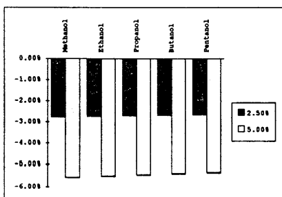
Fig. 5 The change in stoichiometric air to fuel ratio of C 1 -C 5 alcohol-gasoline blends relative to neat gasoline.
