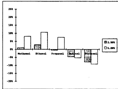
Fig.14 Comparison of alcohol-gasoline blends (2.5% and 5% oxygen mass content)compression ratio to neat gasoline at optimum operation.
