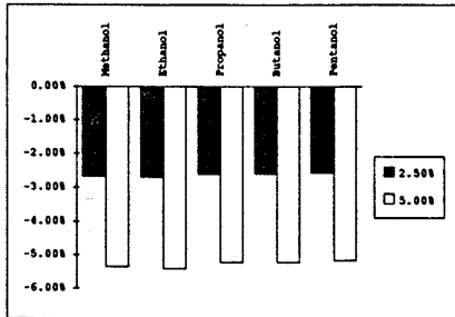
Fig. 3 The change in energy-mass density of C 1 -C 5 alcohol-gasoline blends relative to neat gasoline.
