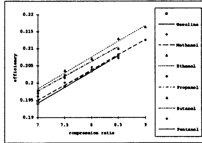
Fig. 9 Maximum brake thermal efficiency at different compression ratios for blends with 5.0% oxygen.
