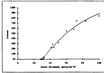
Fig. 6 Percentage of knocking traces versus time averaged knock strength for different operating conditions.
