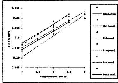
Fig. 8 Maximum brake thermal efficiency at different compression ratios for blends with 2.5% oxygen.
