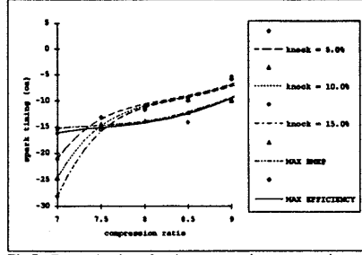
Fig. 7 Determination of optimum operating compression ratio and spark timing.
