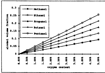
Fig. 1 Alcohol volume fraction in C 1 -C 5 alcohol-gasoline blends with matched oxygen content.
