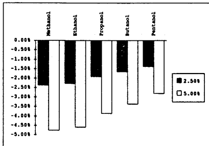
Fig. 4 The change in energy-volume density of C 1 -C 5 alcohol-gasoline blends relative to neat gasoline.
