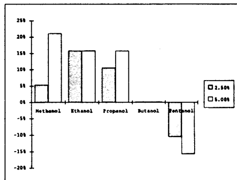
Fig.16 Comparison of alcohol-gasoline blends (2.5% and 5% oxygen mass content) maximum compression ratio to neat gasoline.
