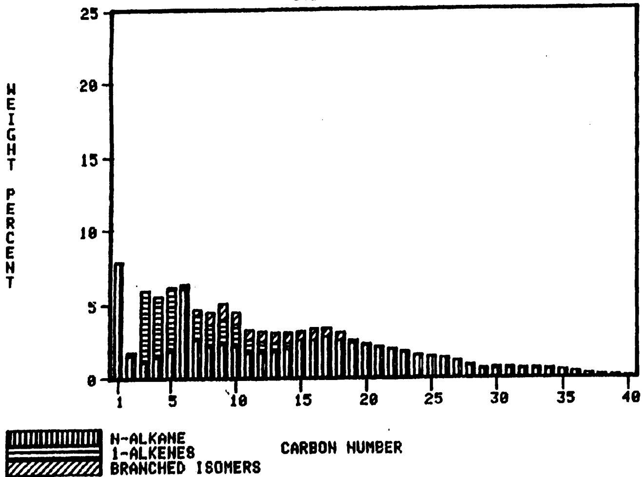
Figure 49 HYDROCARBON WEIGHT DISTRIBUTION 8523-1-4-10
