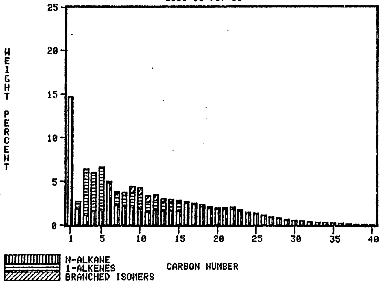
Figure 44 HYDROCARBON WEIGHT DISTRIBUTION 8385-60-787-33
