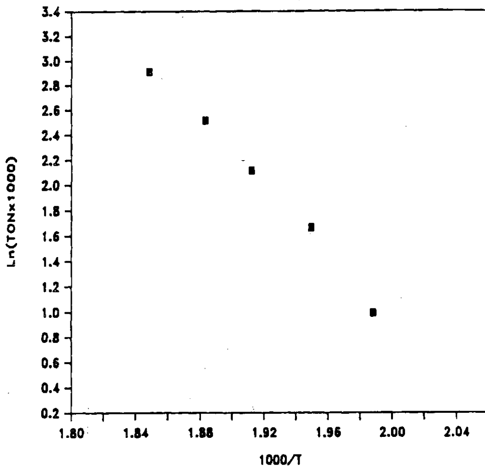
Figure C-6 Arrhenius Plot for CO Hydrogenation on RuCsY
