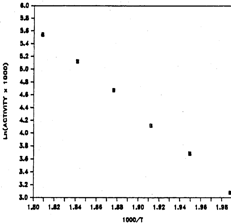
Figure C-9 Arrhenius Plot for CO Hydrogenation on RuKL
