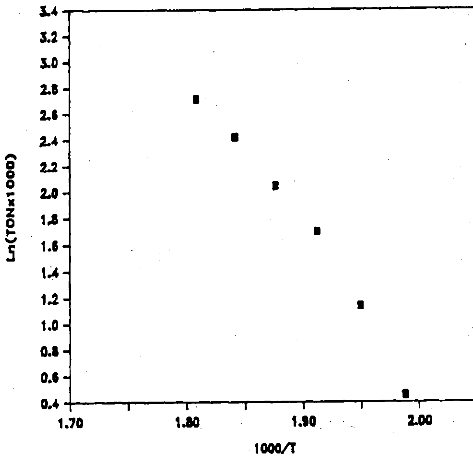
Figure C-4 Arrhenius Plot for CO Hydrogenation on RuKY
