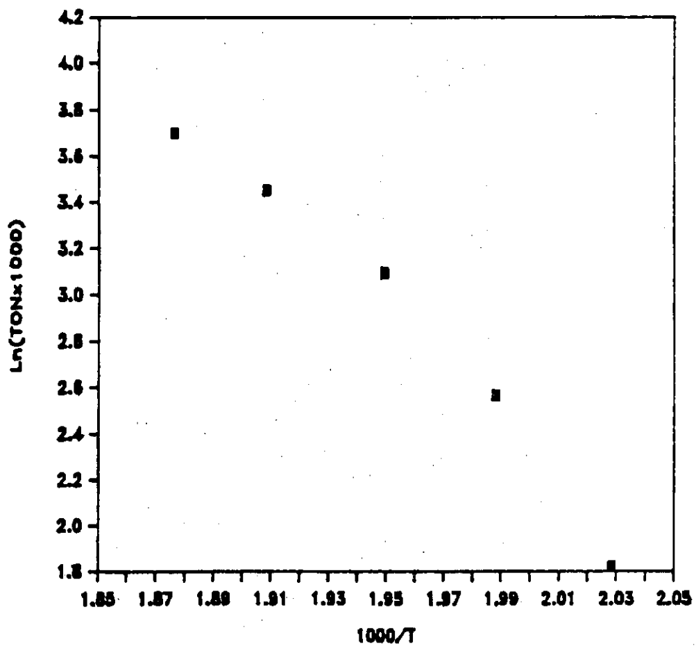
Figure C-1 Arrhenius Plot for CO Hydrogenation on RuHY.
