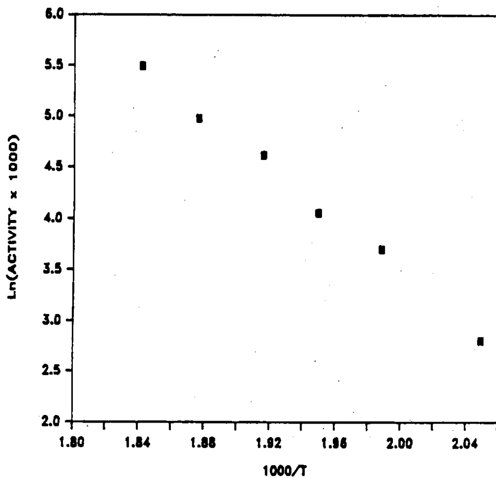
Figure C-7 Arrhenius Plot for CO Hydrogenation on \text{RuSiO}_2
