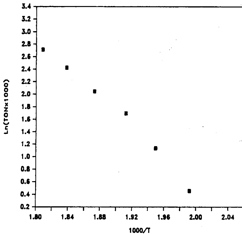
Figure C-5 Arrhenius Plot for CO Hydrogenation on RuRbY
