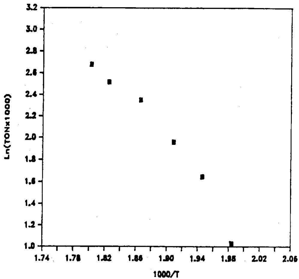
Figure C-3 Arrhenius Plot for CO Hydrogenation on RuNaY
