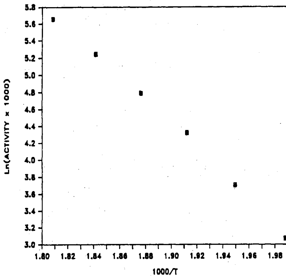
Figure C-10 Arrhenius Plot for CO Hydrogenation on RuNaM
