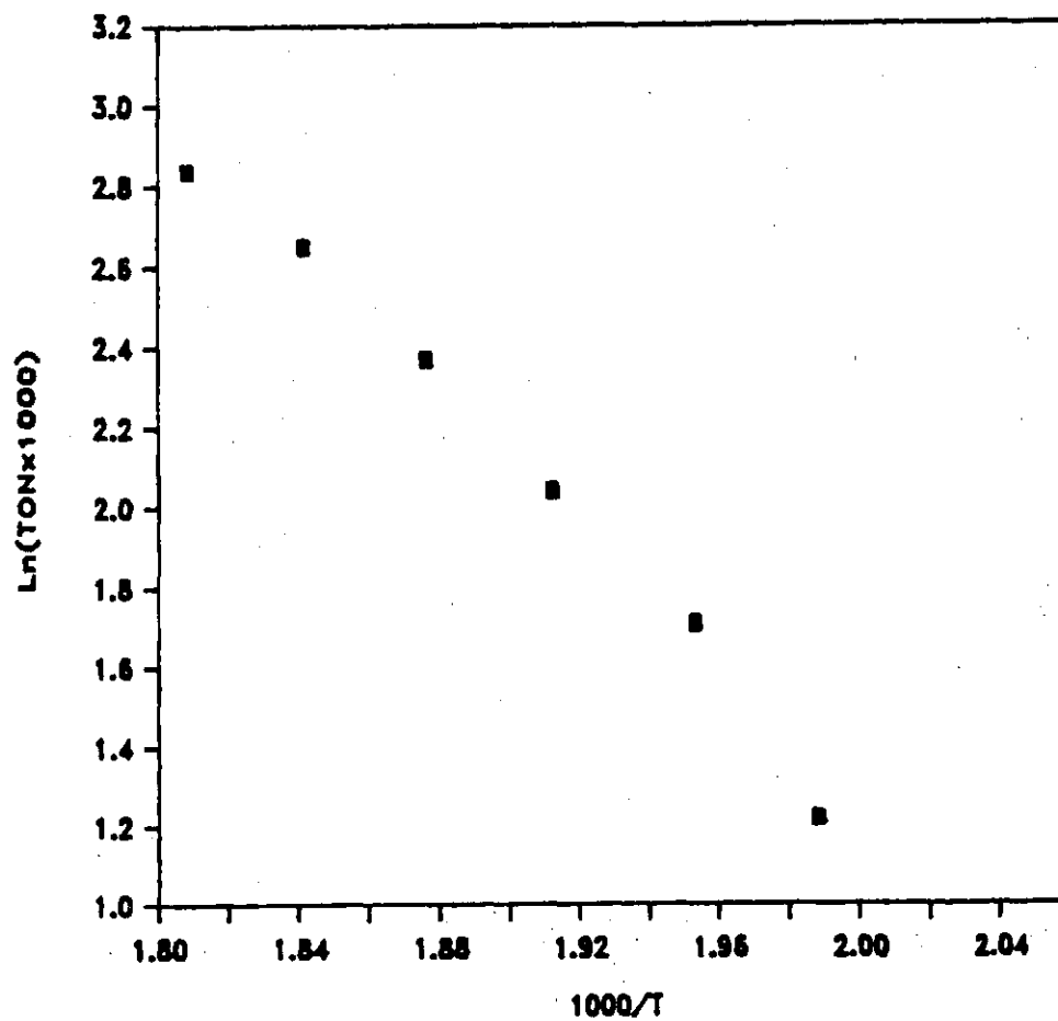
Figure C-2 Arrhenius Plot for CO Hydrogenation on RuLiY
