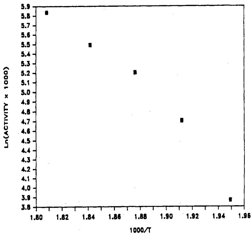
Figure C-8 Arrhenius Plot for CO Hydrogenation on RuNaX
