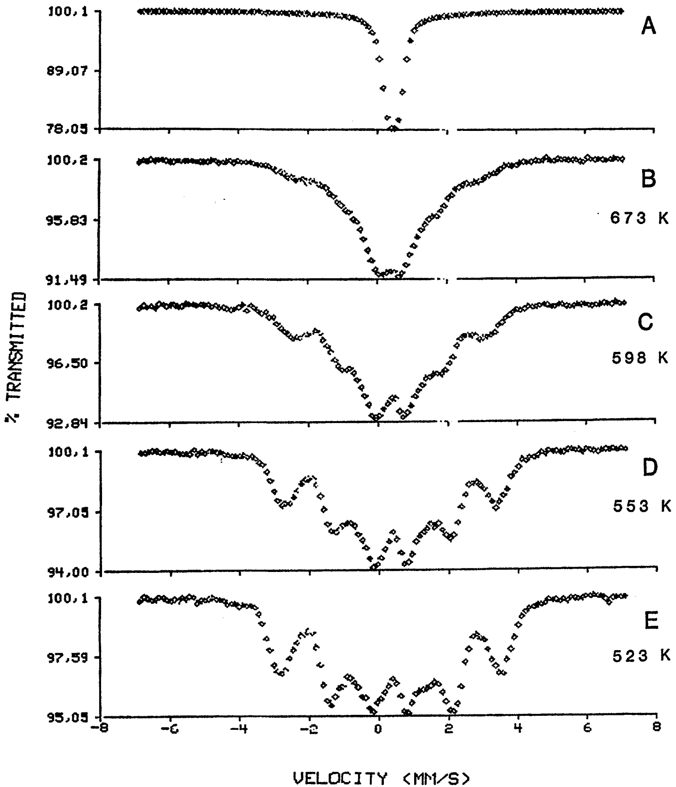
Figure 1: Mössbauer spectra (298 K) of \epsilon -iron nitrides A) Starting \epsilon/\zeta -Fe 2 N then consecutively annealed in 91% NH 3 for 6 hours at respective temperatures (B-E)
