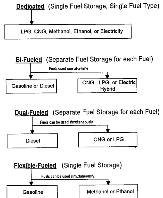
Figure 1. Alternative Fueled Vehicle Configurations and Fuel Types
